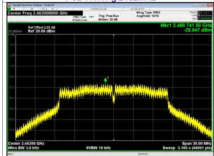
PSD NVNT g 2462MHz
