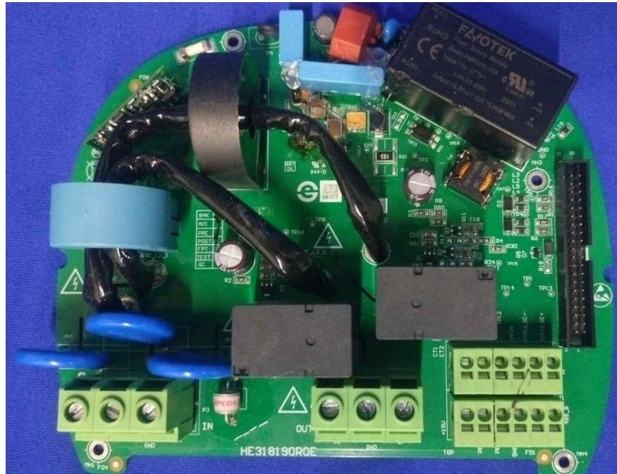
Power Card Top View:
