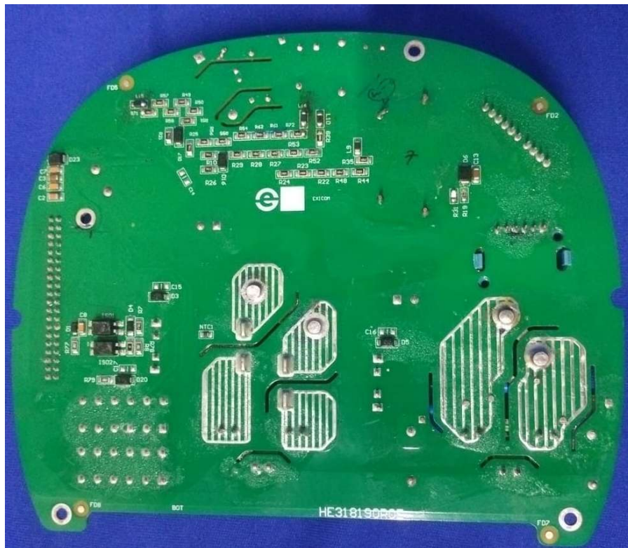
Power Card Bottom View
