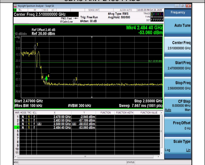
3D5-Ant1-Hop_2480-PASS
