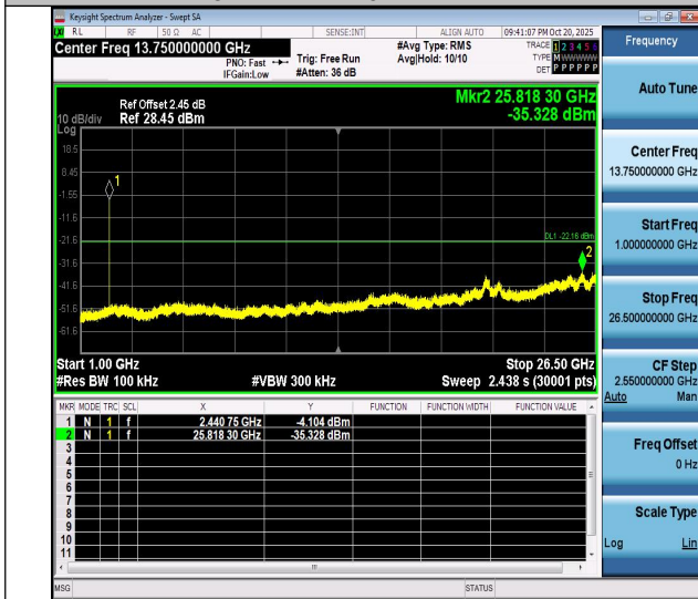
2DH5-Ant1-2441-1000~26500-PASS
