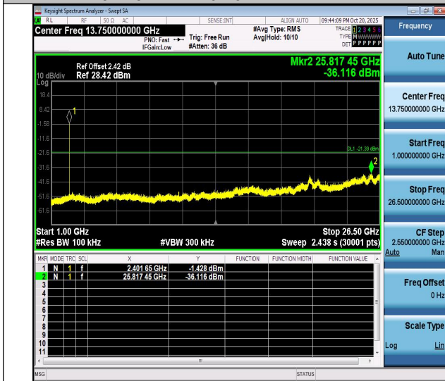
3DH5-Ant1-2402-1000~26500-PASS
