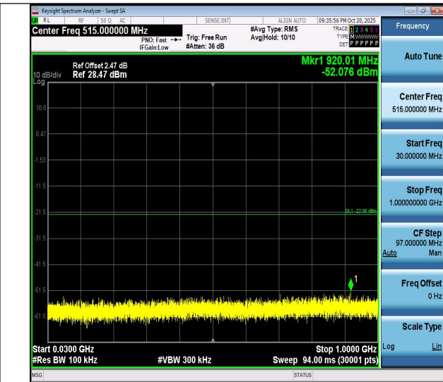
DH5-Ant1-2480-30~1000-PASS
