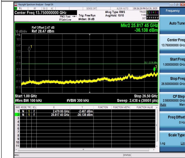
DH5-Ant1-2480-1000~26500-PASS
