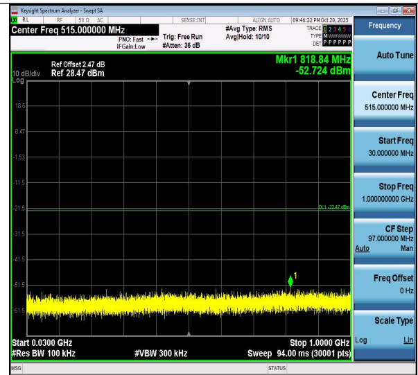
3DH5-Ant1-2480-30~1000-PASS
