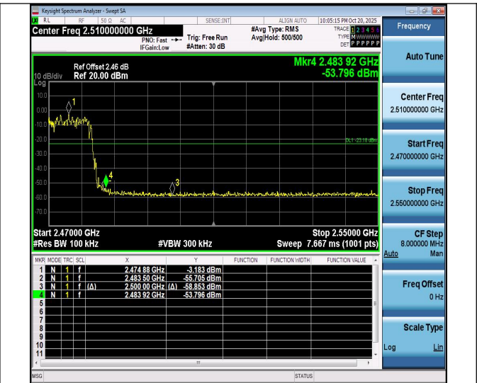
2D5-Ant1-Hop_2480-PASS
