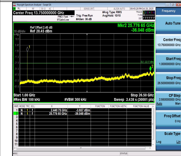
3DH5-Ant1-2441-1000~26500-PASS
