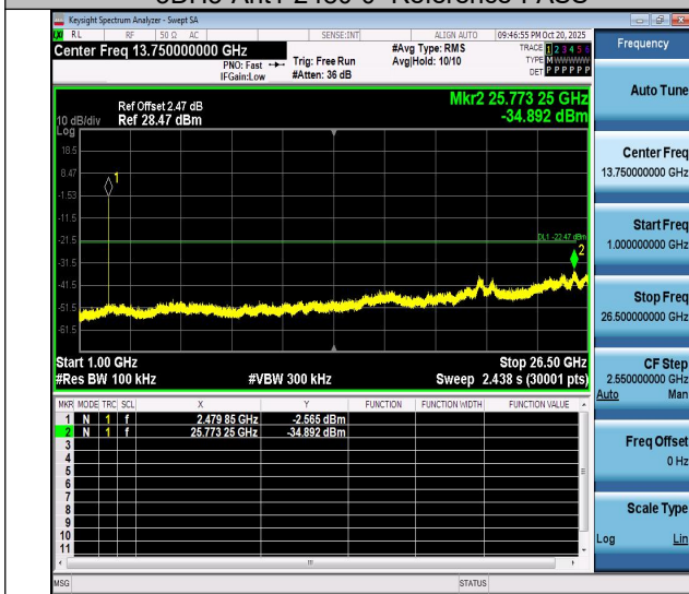
3DH5-Ant1-2480-1000~26500-PASS
