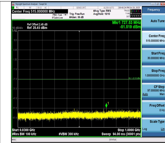
2DH5-Ant1-2441-30~1000-PASS
