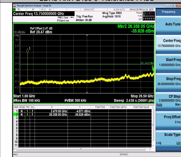
2DH5-Ant1-2480-1000~26500-PASS
