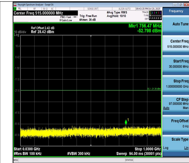
3DH5-Ant1-2402-30~1000-PASS
