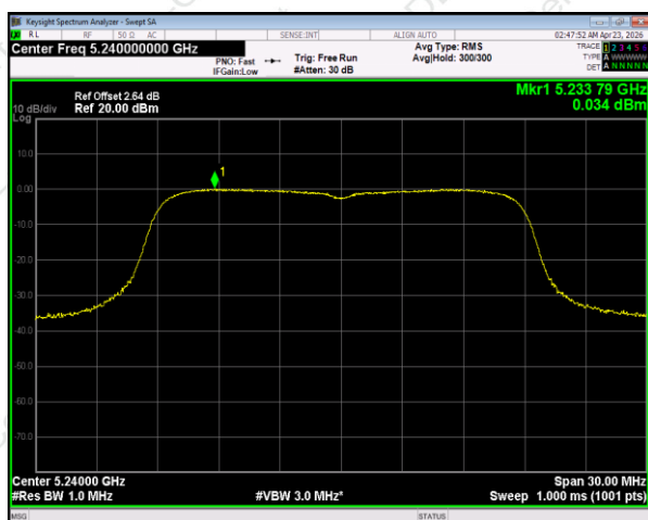
(802.11ac20) PSD plot on channel 48
