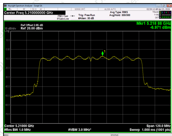
(802.11ac80) PSD plot on channel 42
