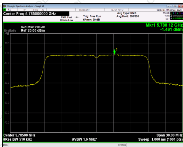
(802.11n20) PSD plot on channel 157
