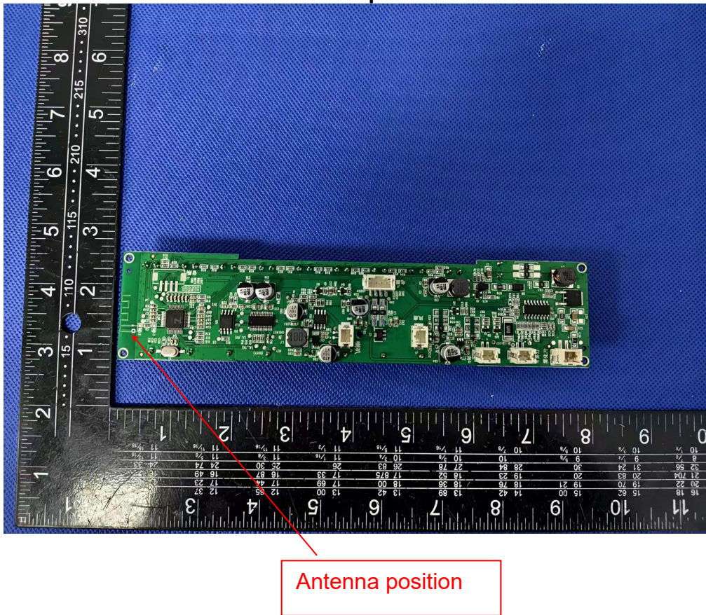
Photo 3 Internal photos of EUT
