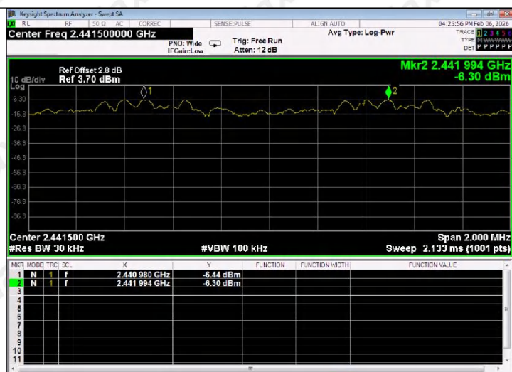
8-DPSK
