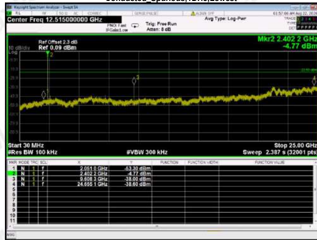
Conducted_Spurious,1DH5,Lowest
