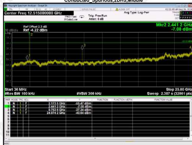
Conducted_Spurious,2DH5,Middle
