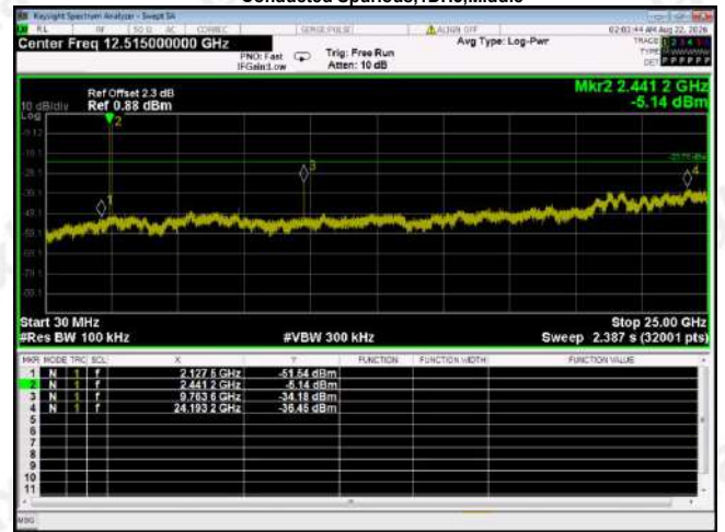
Conducted Spurious,1DH5,Middle
