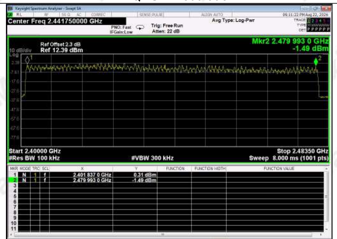
8-DPSK Modulation
