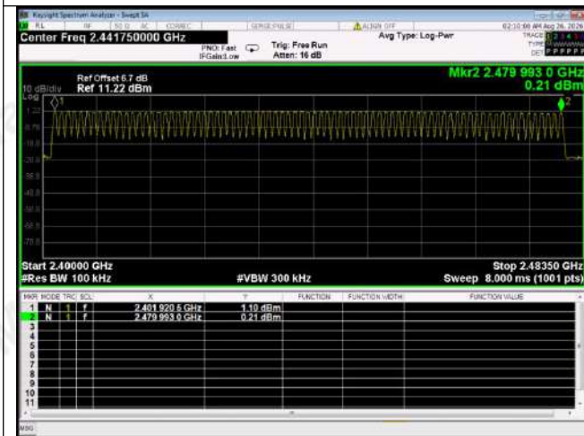
GFSK Modulation
