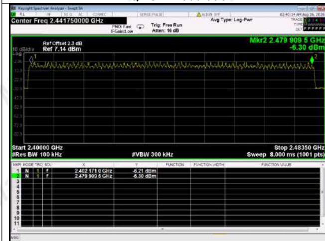
8-DPSK Modulation
