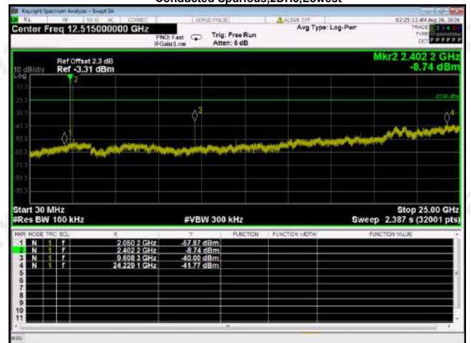
Conducted Spurious,2DH5,Lowest
