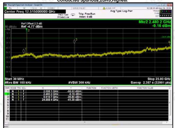
Conducted Spurious,2DH5,Highest
