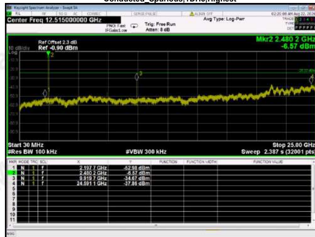
Conducted_Spurious,1DH5,Highest
