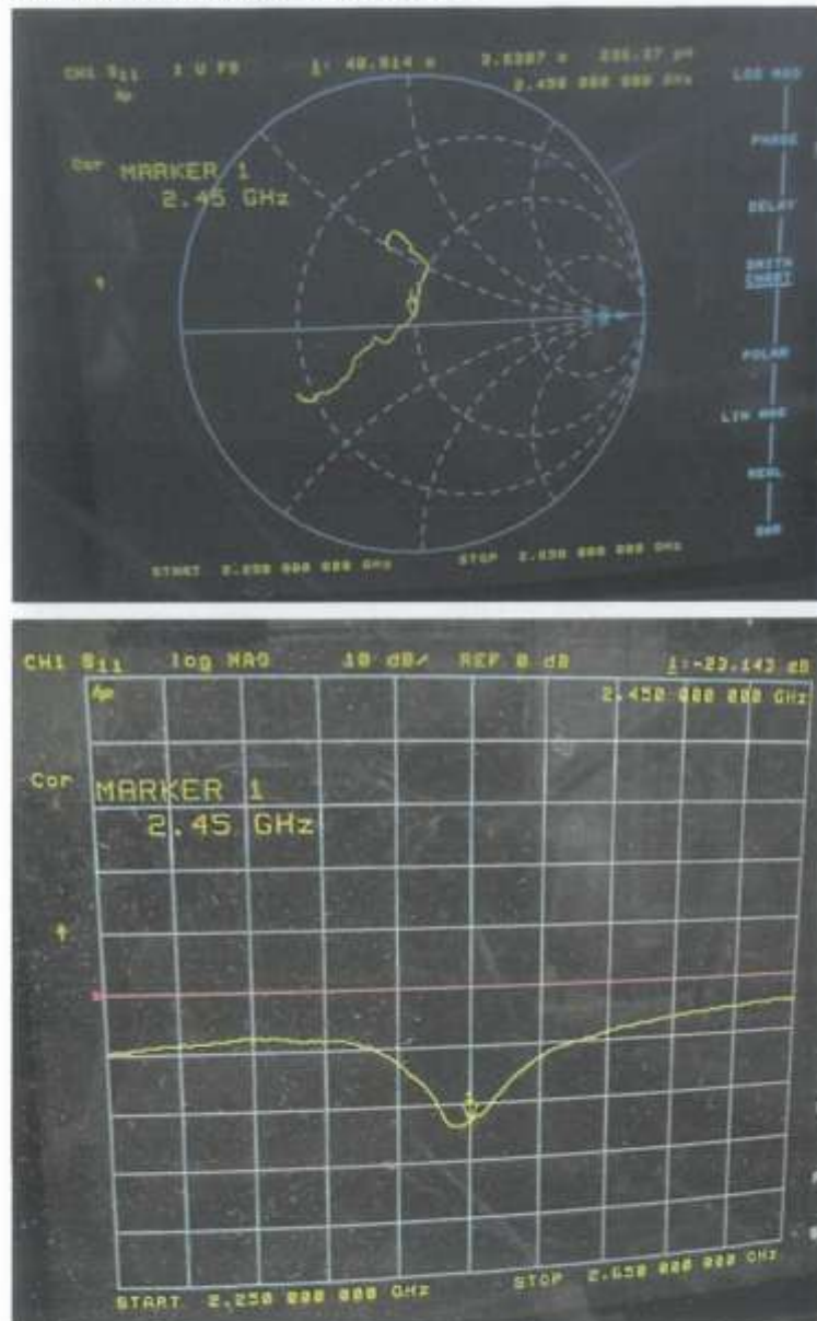
Impedance & Return-Loss Measurement Plot for Head TSL
