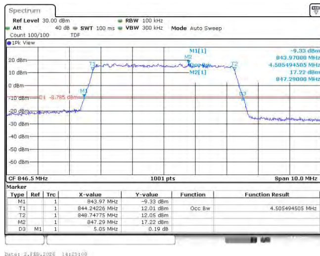
Band26-5MHz-16QAM-26815-25RB#0-4.505
