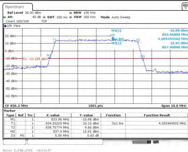
Band26-5MHz-16QAM-27015-25RB#0-4.505
