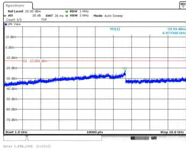
Band26-5MHz-QPSK-26740-25RB#0-Range1:30~1000MHz
