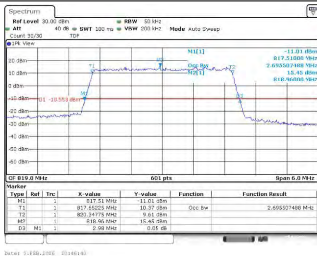
Band26-3MHz-16QAM-26775-15RB#0-2.696
