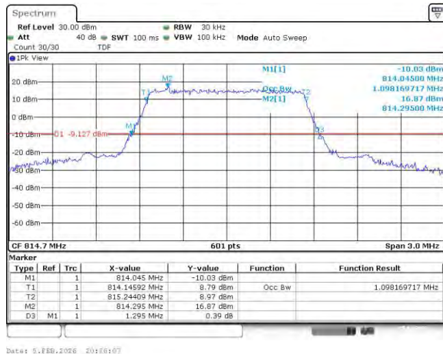
Band26-1.4MHz-16QAM-26740-6RB#0-1.098
