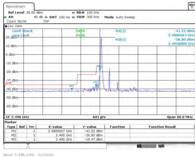
Band41-5MHz-16QAM-39675-1RB#24
