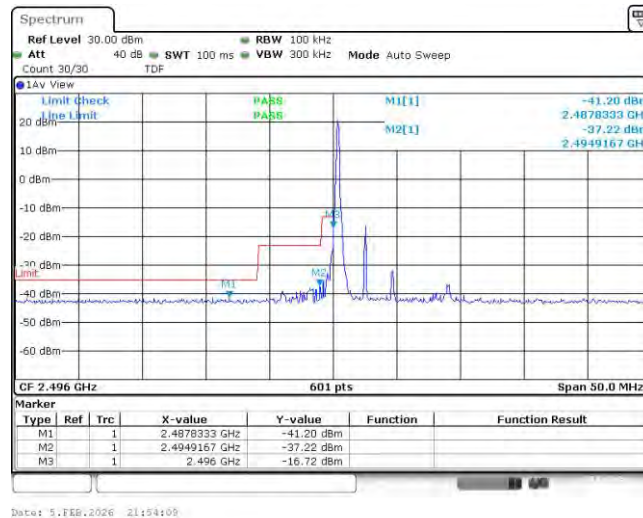
Band41-5MHz-QPSK-39675-1RB#24
