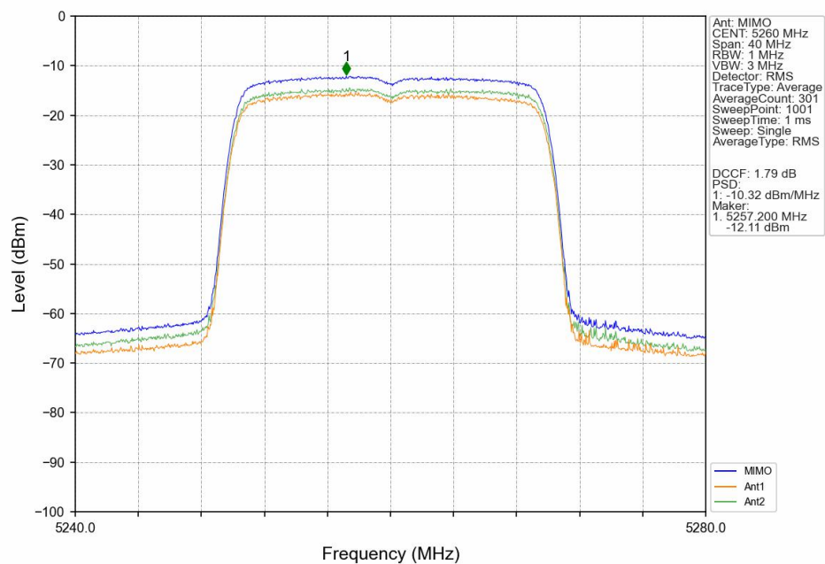
802.11ax(HEW20)_LCH_5260MHz_SU_ / MIMO_NTNV
