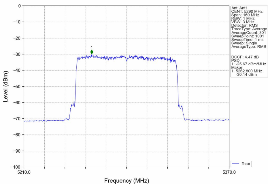
802.11ax(HEW80)_MCH_5290MHz_SU_ / Ant1_NTNV
