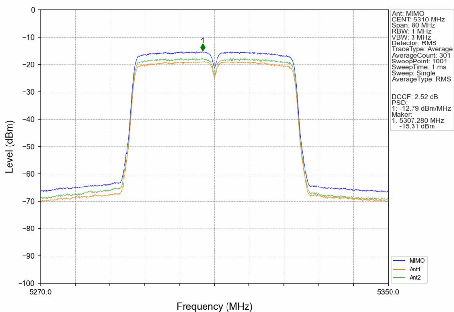
802.11ac(VHT40)_HCH_5310MHz_MIMO_NTNV
