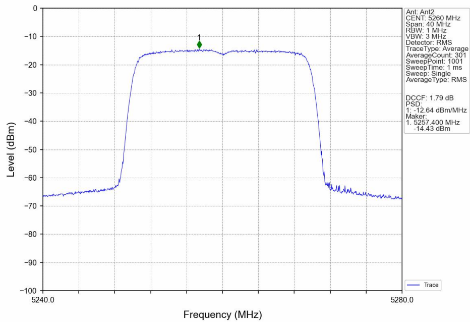
802.11ax(HEW20)_LCH_5260MHz_SU_ / MIMO_NTNV
