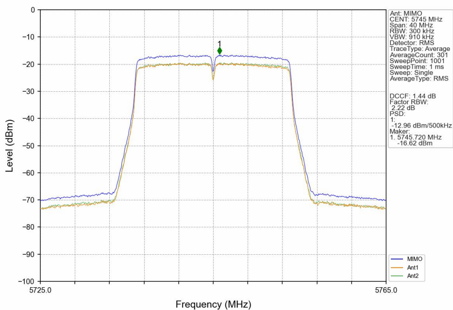
802.11ac(VHT20) LCH_5745MHz_MIMO_NTNV
