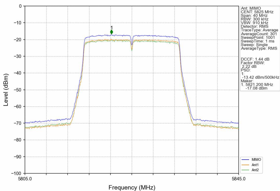
802.11ac(VHT20)_HCH_5825MHz_MIMO_NTNV
