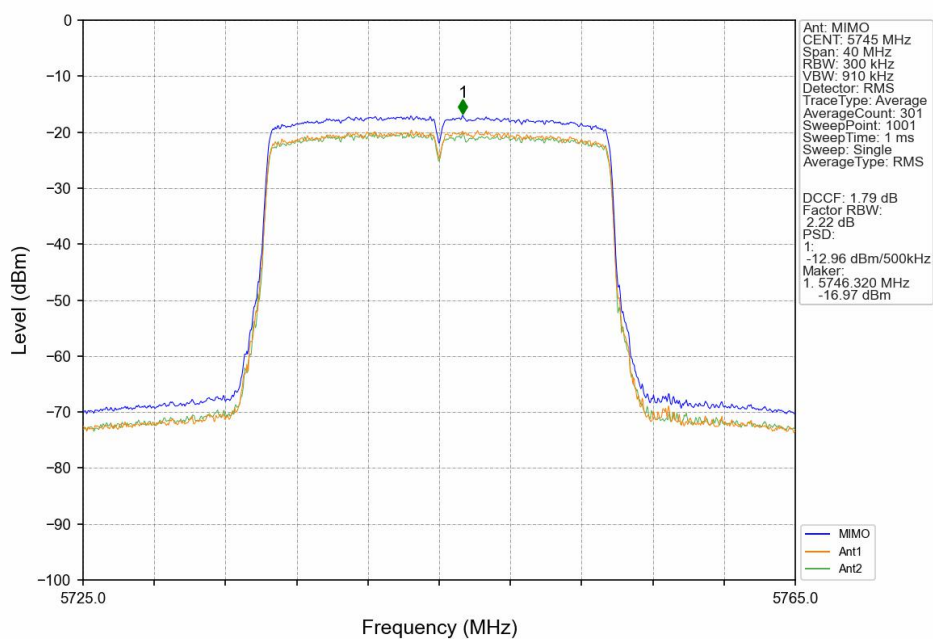
802.11ax(HEW20)_LCH_5745MHz_SU_ / MIMO_NTNV
