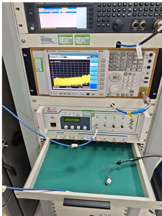
Conducted Emission Test View
