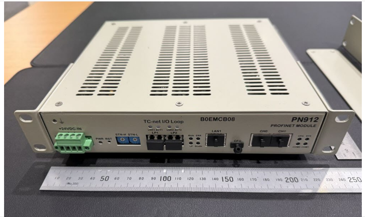
Figure 1 – PN912 Front View
