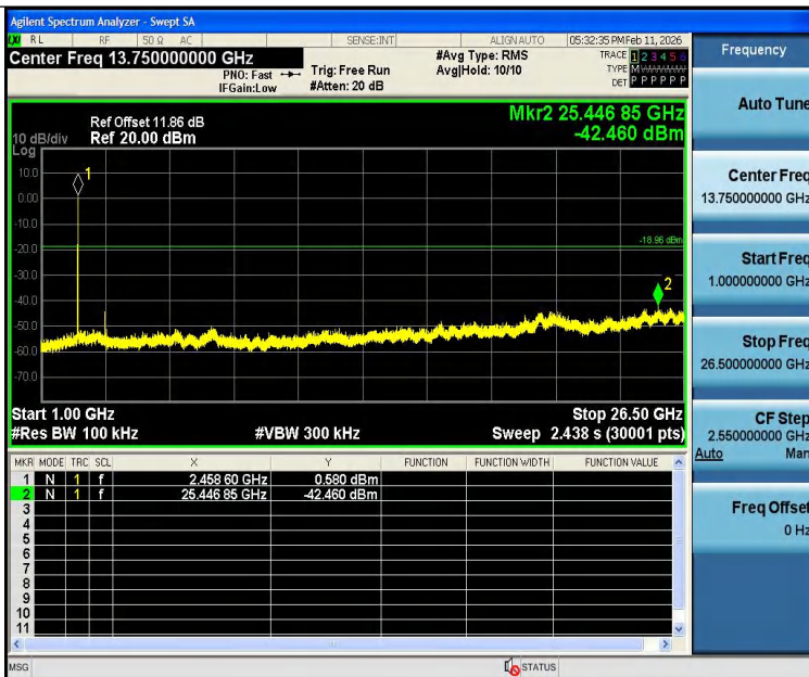
11G-Ant1-2412-0~Reference-PASS
