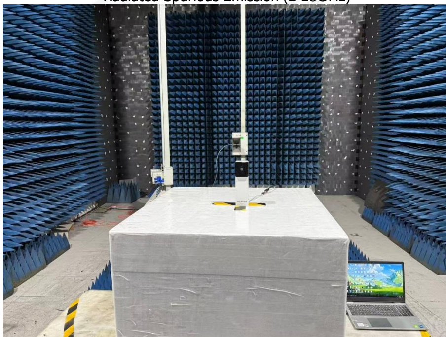
Radiated Spurious Emission (1-18GHz)
