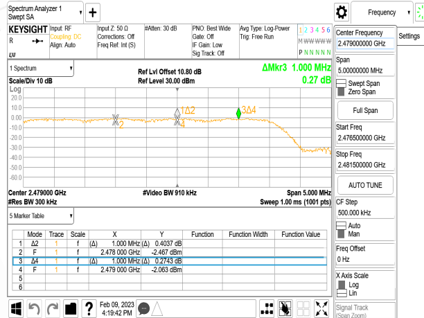
\pi/4 DQPSK_2M_DH5_CH76CH77CH78
