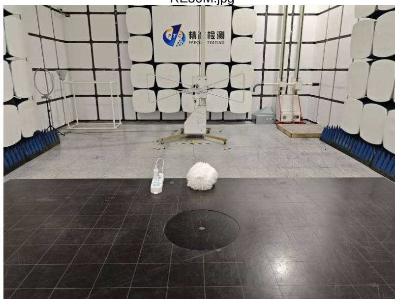
Radiated Spurious Emissions From 30MHz-1000MHz RE30M.jpg
