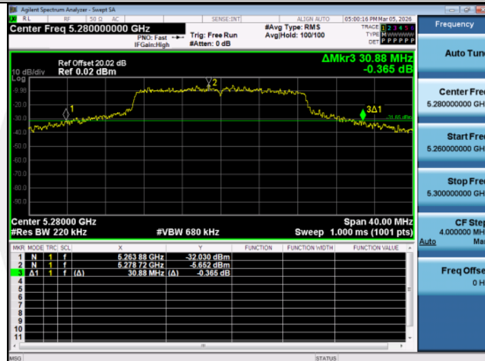
11AC20SISO-Ant1-5280
