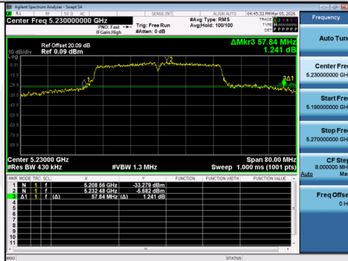
11N40SISO-Ant1-5230
