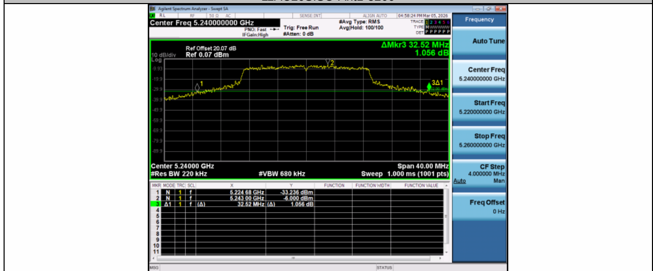
11AC20SISO-Ant1-5240
