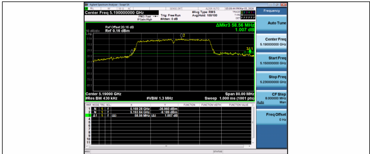
11AC40SISO-Ant1-5190
