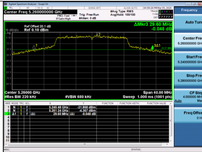
11AC20SISO-Ant1-5260
