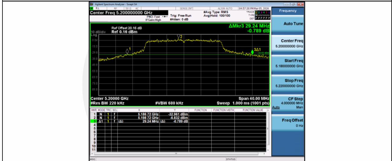
11AC20SISO-Ant1-5200
