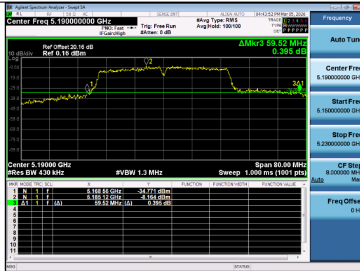
11N40SISO-Ant1-5190
