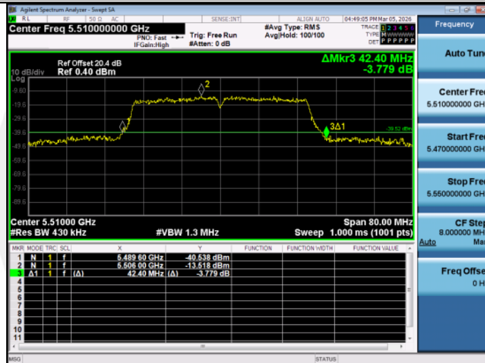
11N40SISO-Ant1-5510
