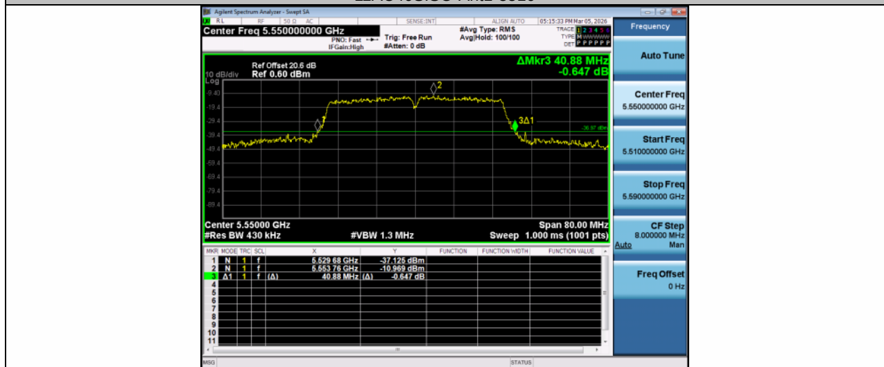
11AC40SISO-Ant1-5550
