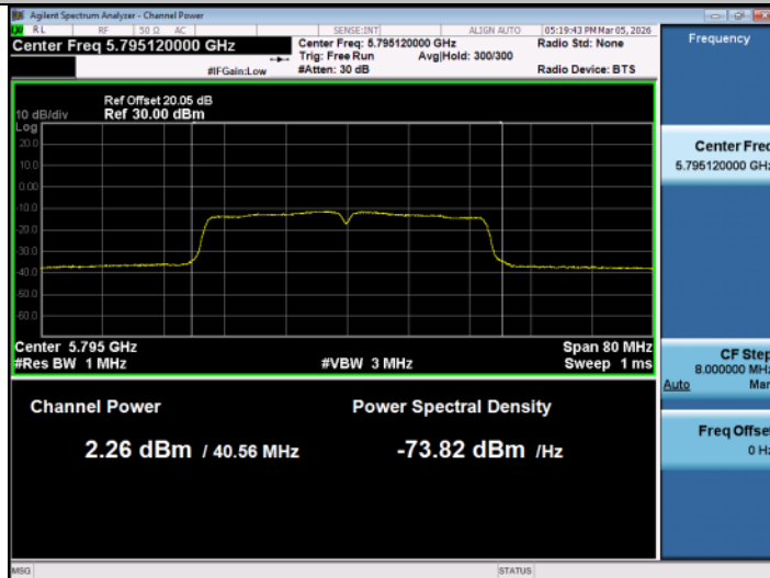
11AC40SISO-Ant1-5795-PASS
