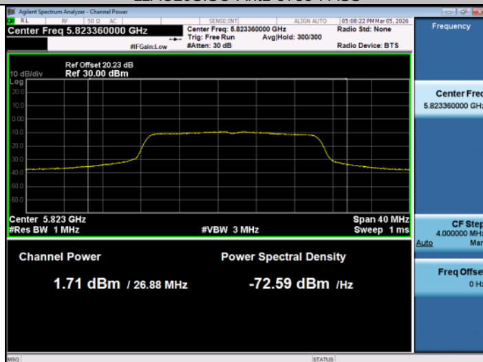
11AC20SISO-Ant1-5825-PASS
