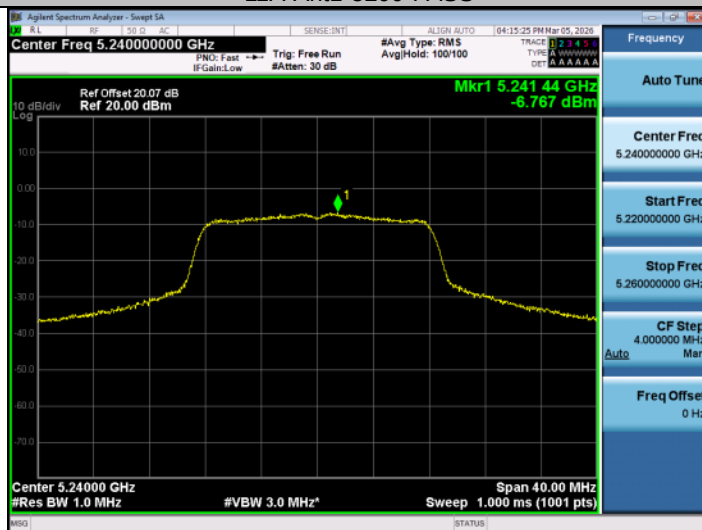
11A-Ant1-5240-PASS
