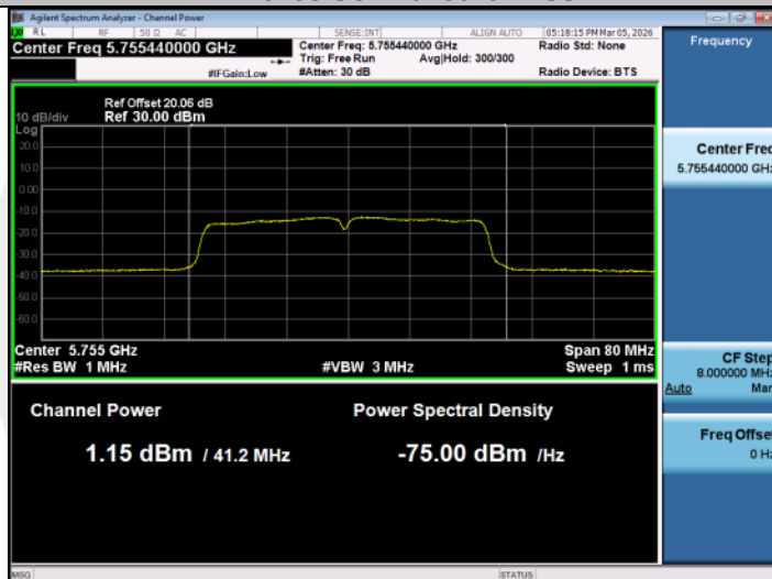
11AC40SISO-Ant1-5755-PASS
