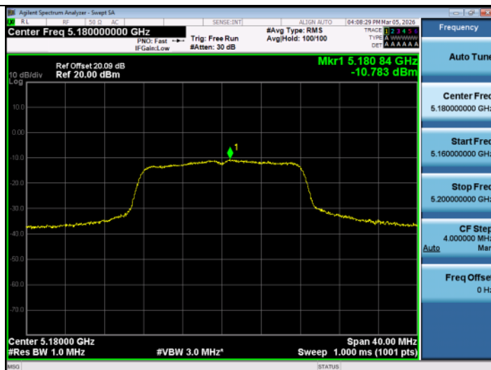
11A-Ant1-5180-PASS
