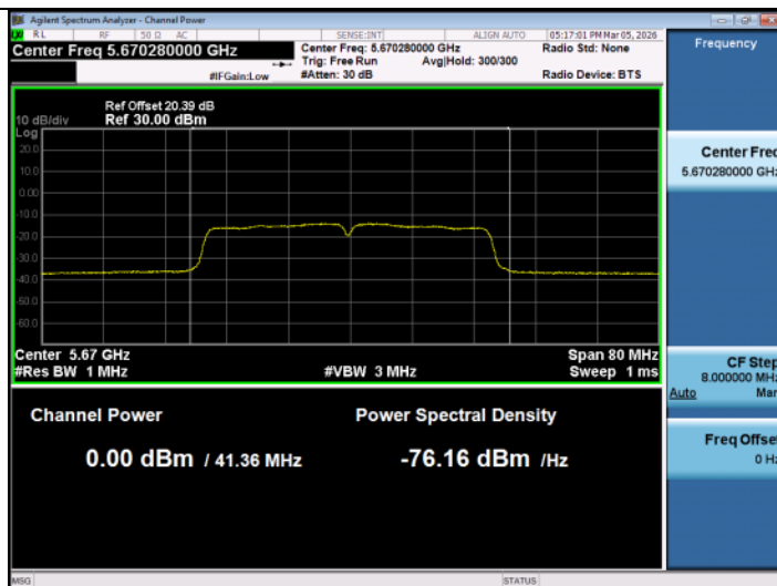
11AC40SISO-Ant1-5670-PASS
