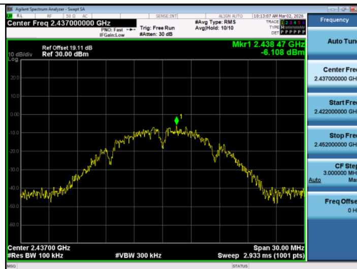
11B-Ant1-2437-0~Reference-PASS
