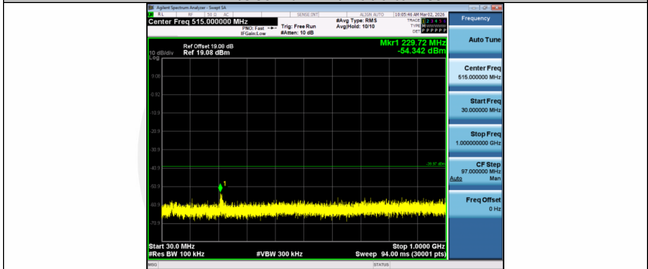
11N40SISO-Ant1-2422-30~1000-PASS
