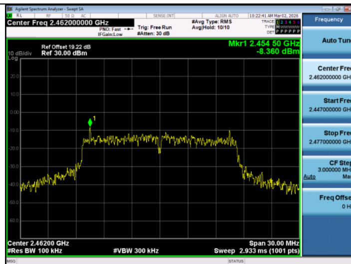
11G-Ant1-2462-0~Reference-PASS
