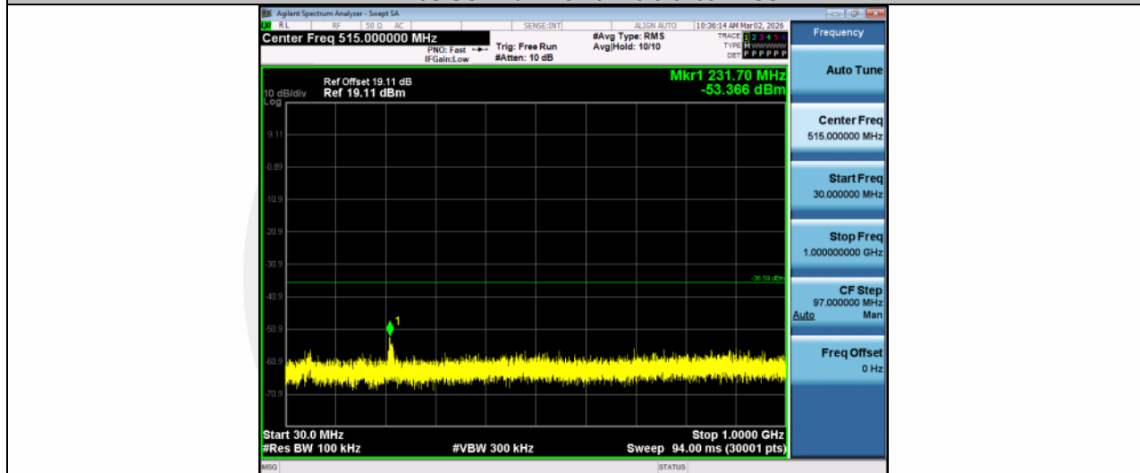
11N20SISO-Ant1-2437-30~1000-PASS
