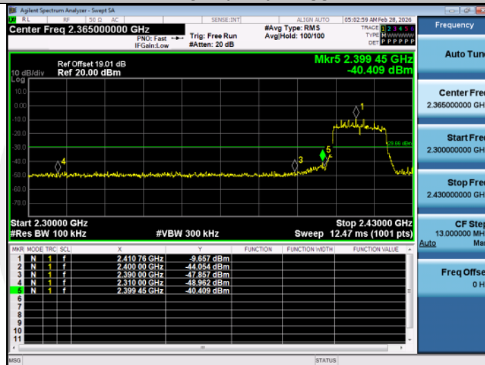
11N20SISO-Ant1-2412-PASS
