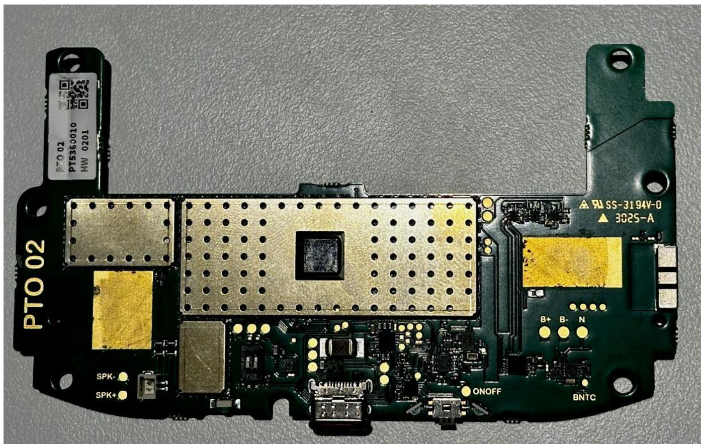
Picture 8 Internal pictures PCB Top view with shield, photo provided by customer
