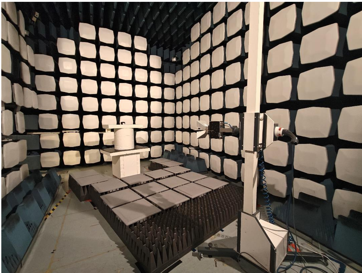
Picture 12 Radiated emission pictures 1 – 18GHz
