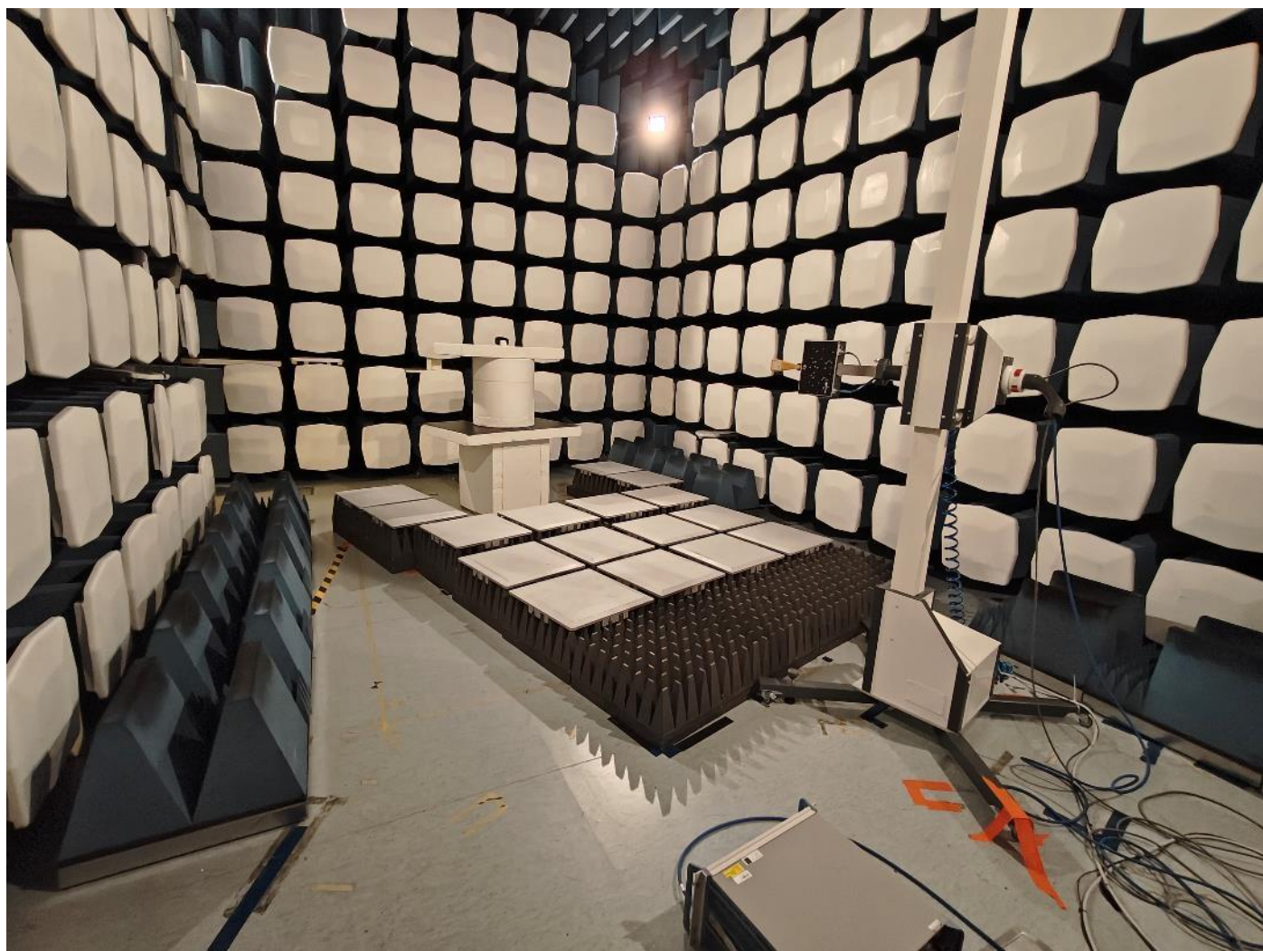
Picture 15 Radiated emission pictures 18 – 26 GHz
