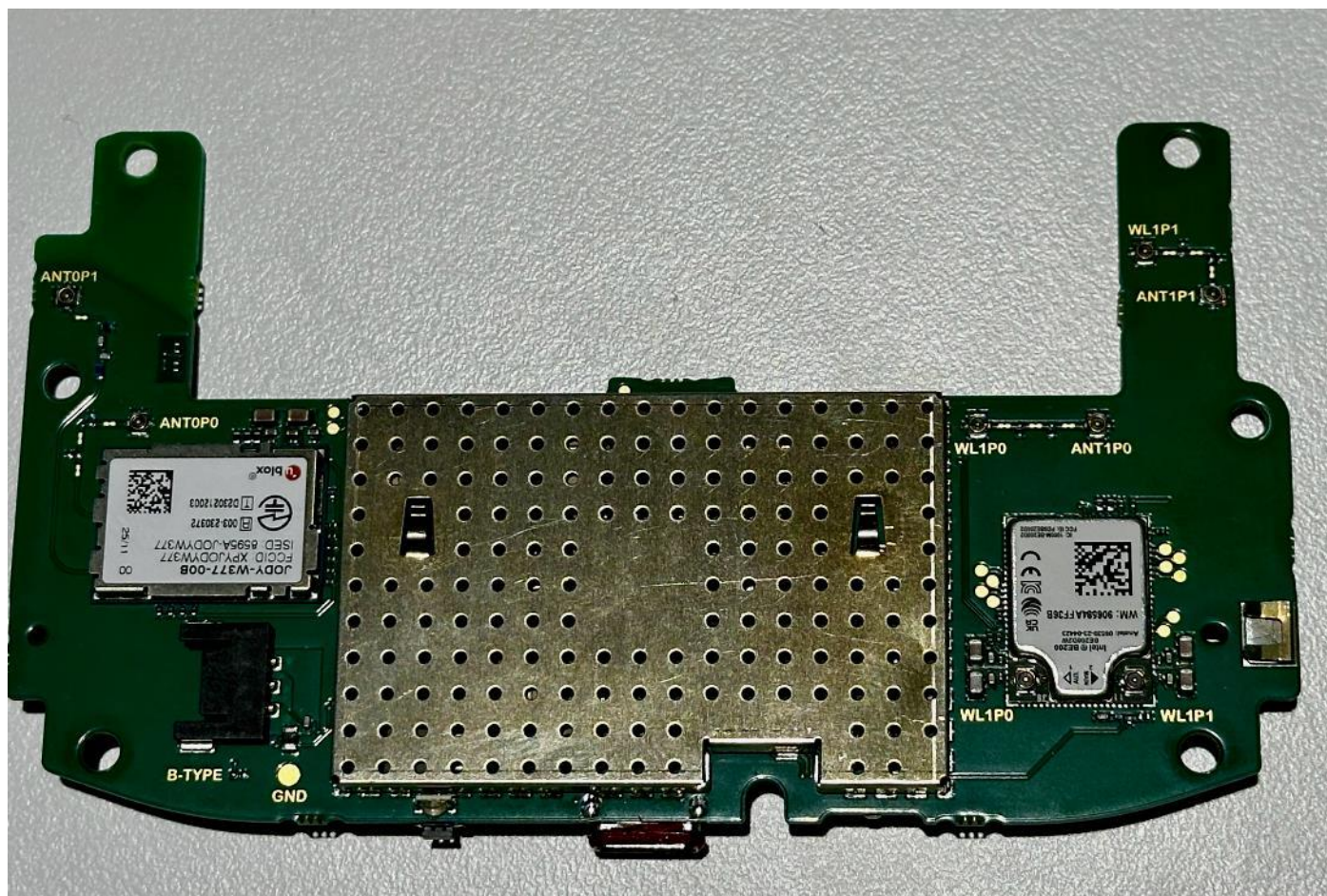
Picture 7 Internal pictures PCB Bottom view with shield, photo provided by customer
