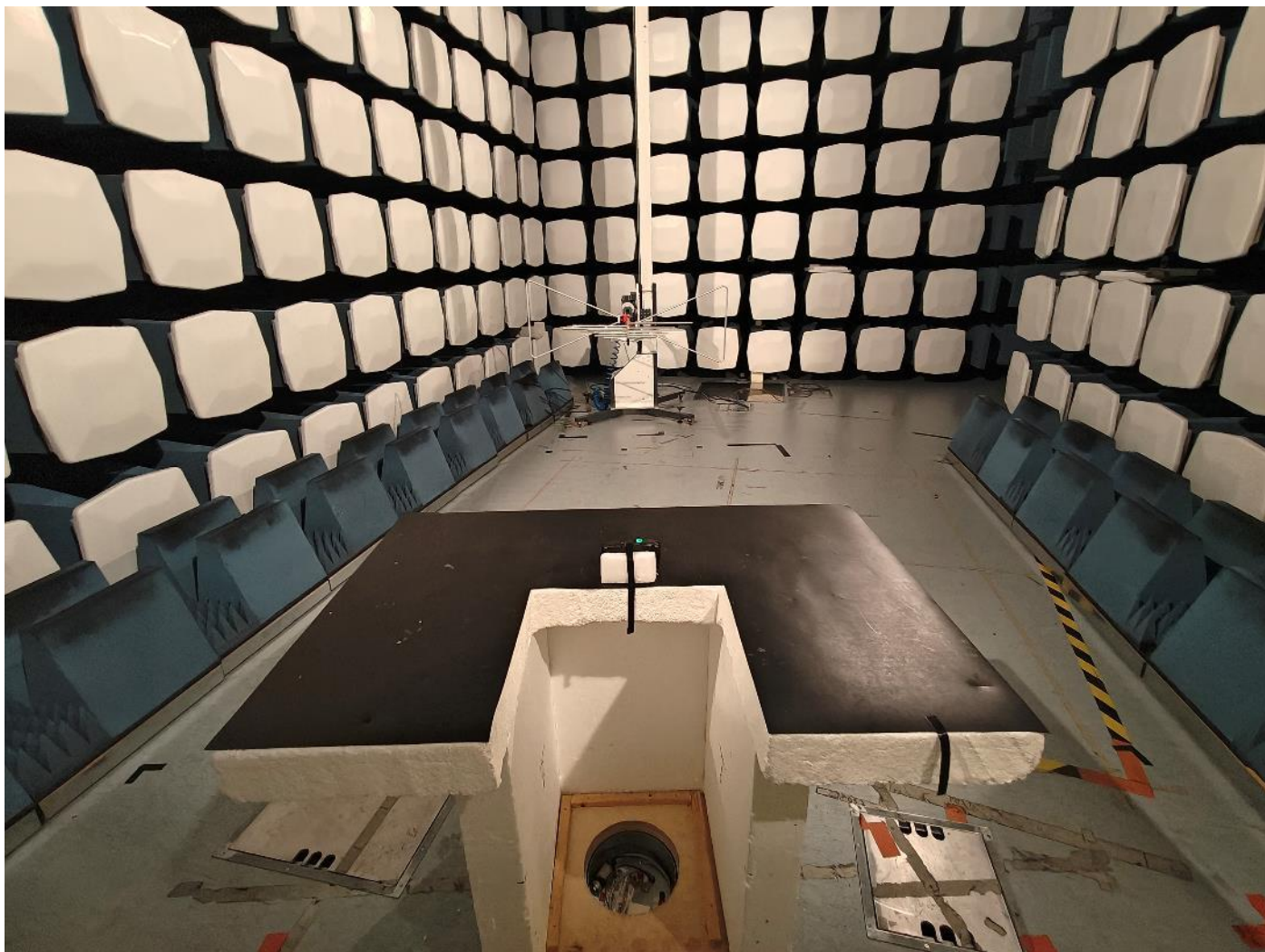
Picture 11 Radiated emission pictures 30-1000MHz
