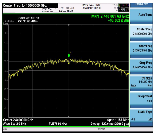
LE_2M-Ant1-2440-PASS
