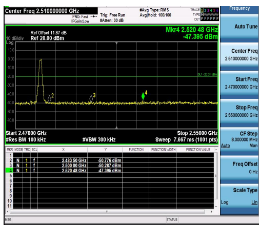
LE_2M-Ant1-2480-PASS
