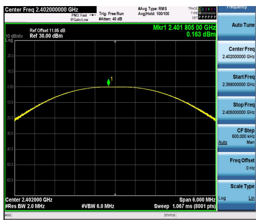
LE_2M-Ant1-2402-PASS
