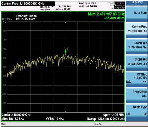
LE_1M-Ant1-2480-PASS
