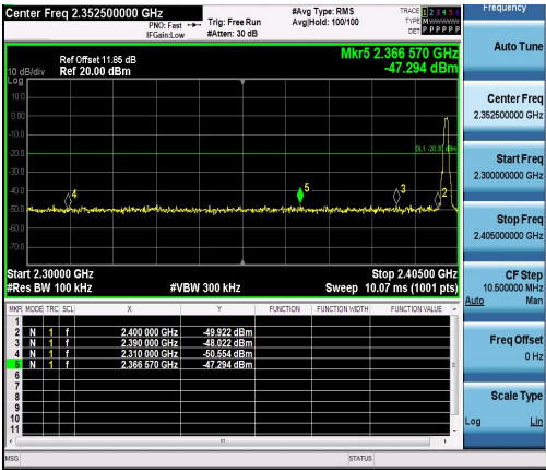
LE_2M-Ant1-2402-PASS
