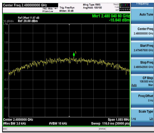
LE_2M-Ant1-2480-PASS
