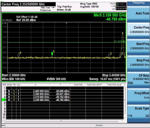
LE_1M-Ant1-2402-PASS
