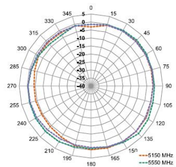
XY-Plane Gain
