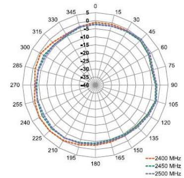
XY-Plane Gain
