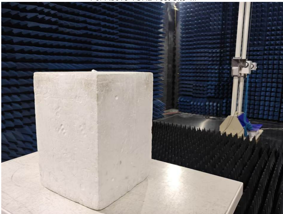
Right Earbud For 9kHz-30MHz Test Site 2#
