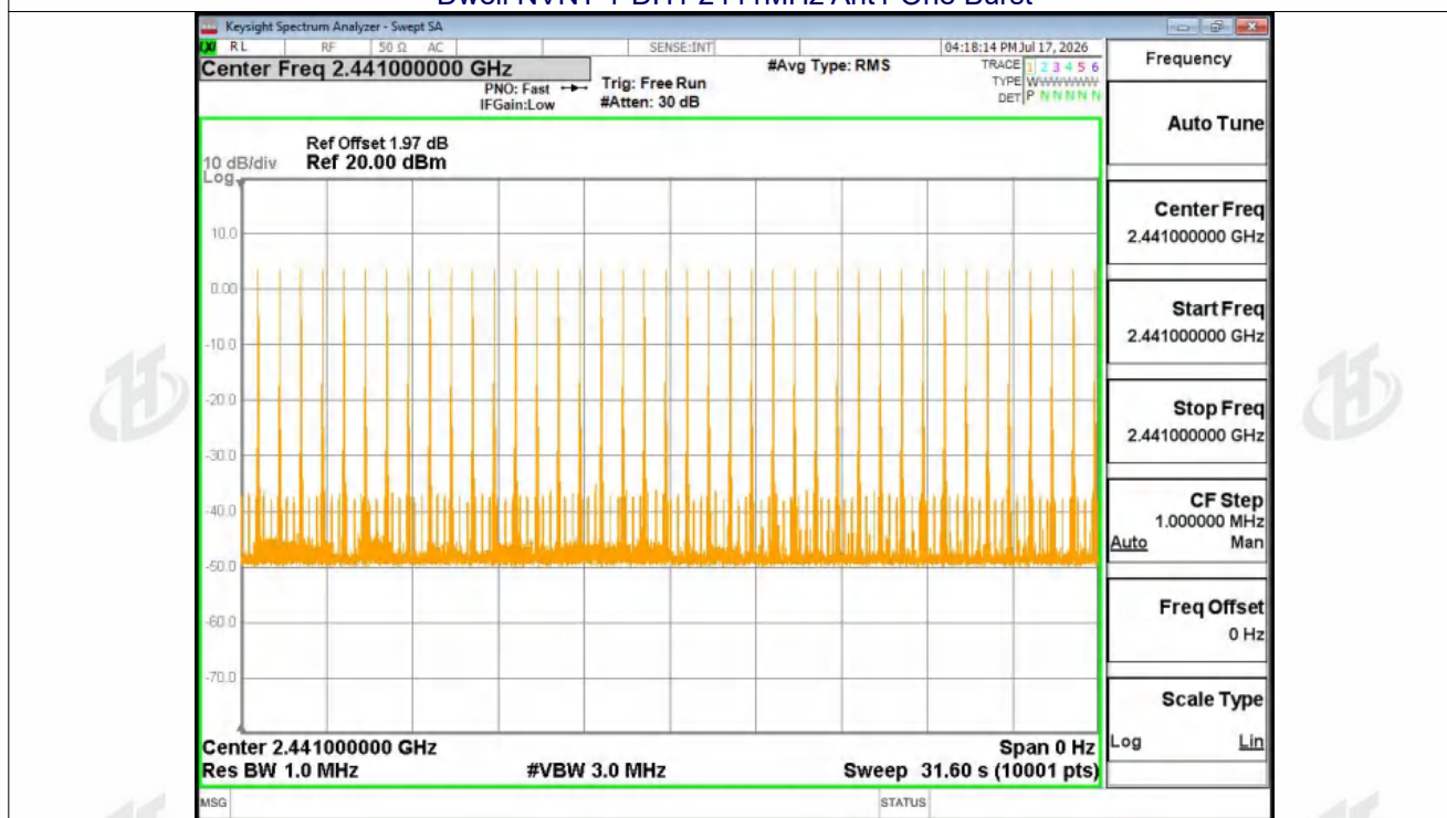
Dwell NVNT 1-DH1 2441MHz Ant1 Accumulated
