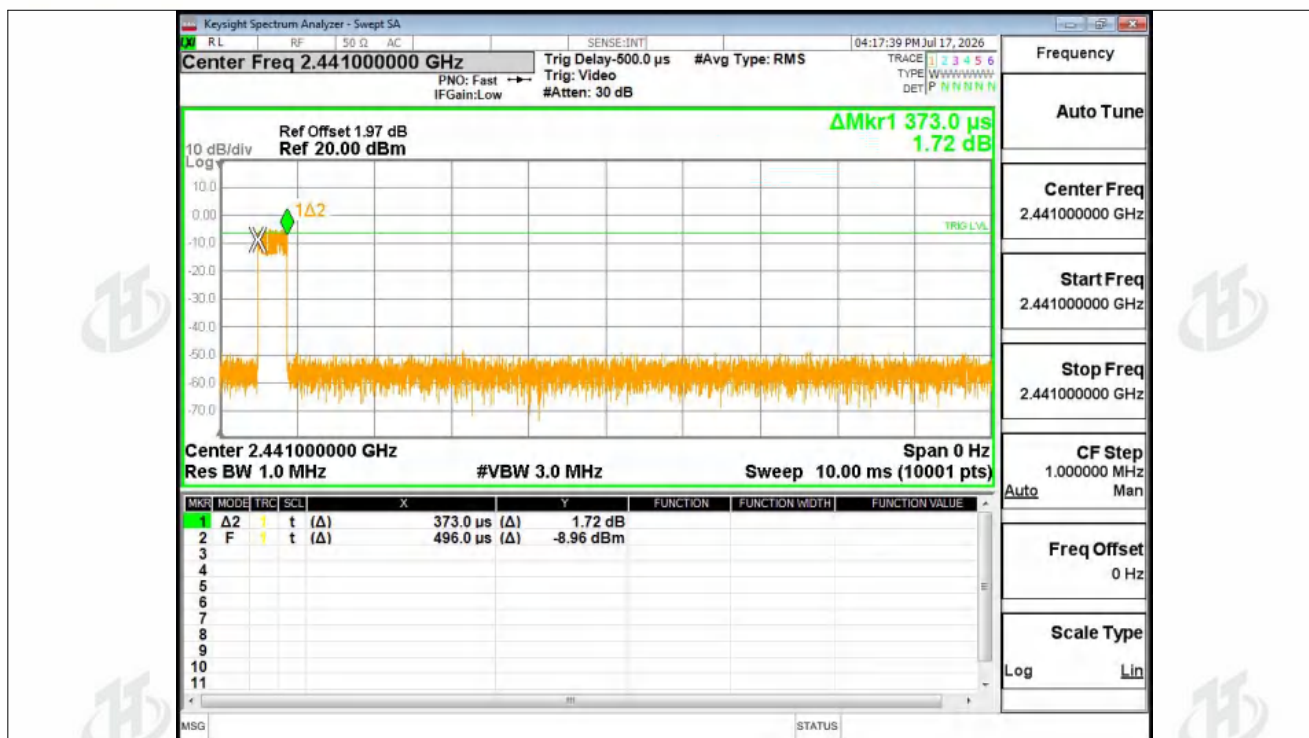
Dwell NVNT 1-DH1 2441MHz Ant1 One Burst
