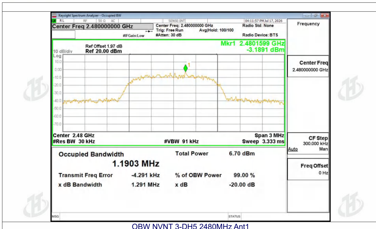
OBW NVNT 3-DH5 2480MHz Ant1
