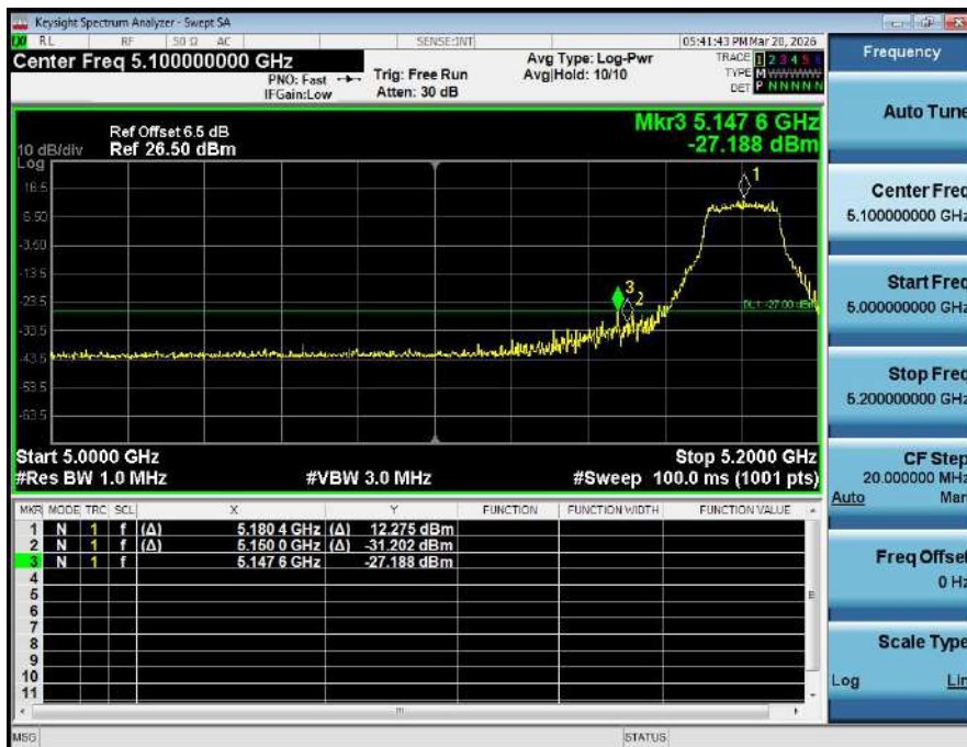
Bandedge_NVNT_ANT1_802_11ax(HE20)_5180
