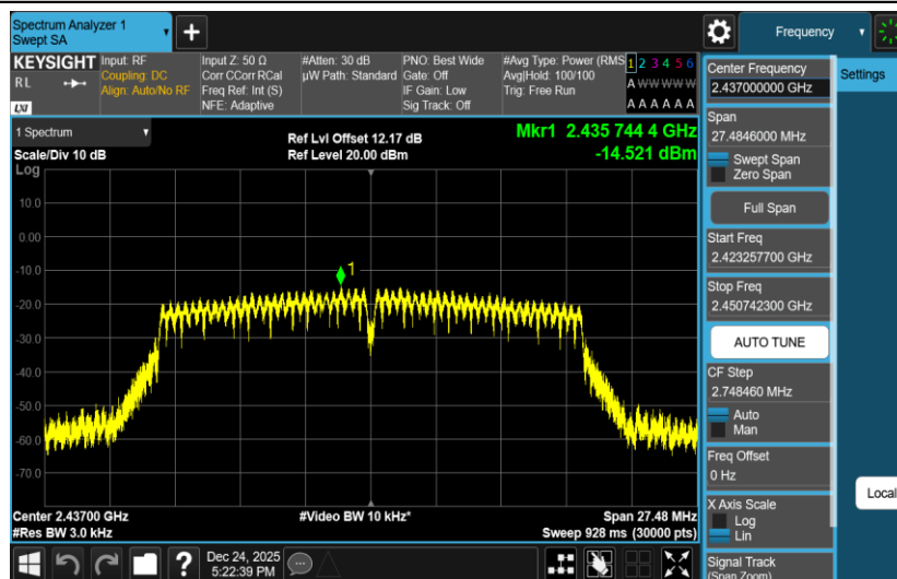
11N20SISO-Ant2-2437-PASS
