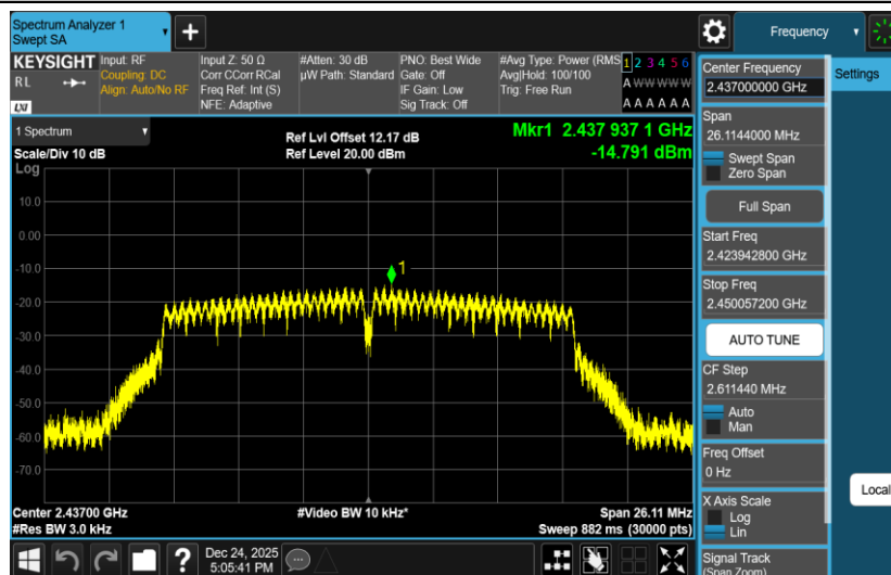
11G-Ant2-2437-PASS
