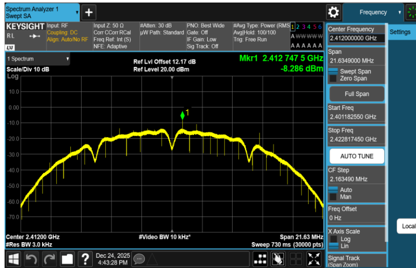
11B-Ant2-2412-PASS
