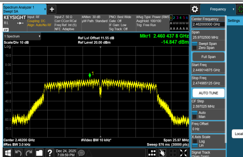
11N20SISO-Ant1-2412-PASS
