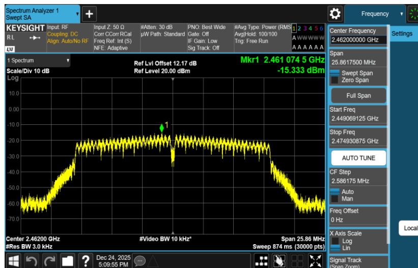
11G-Ant2-2462-PASS
