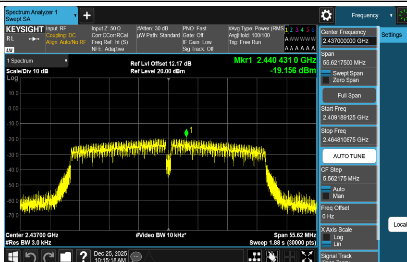
11N40MIMO-Ant2-2437-PASS
