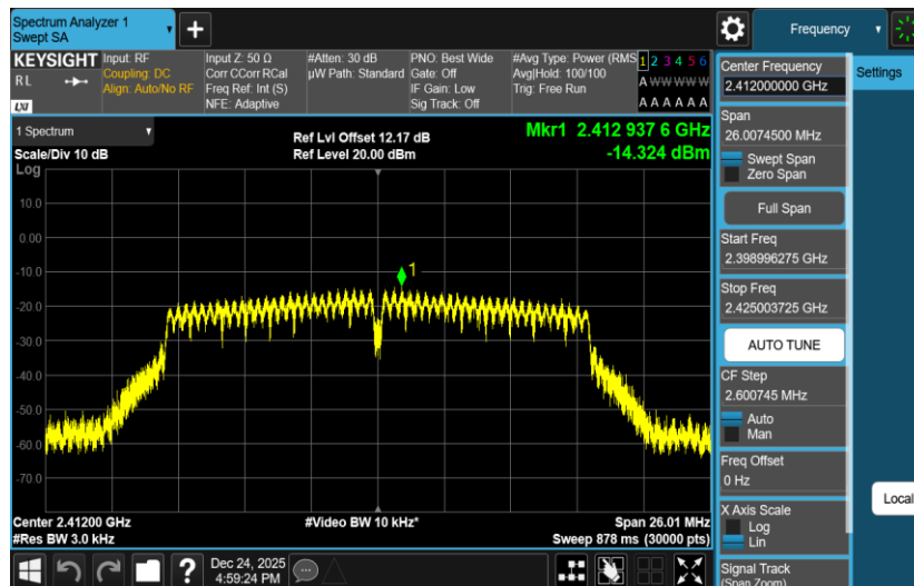
11G-Ant2-2412-PASS
