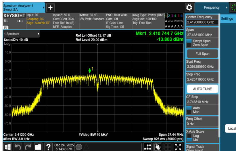
11N20SISO-Ant2-2412-PASS
