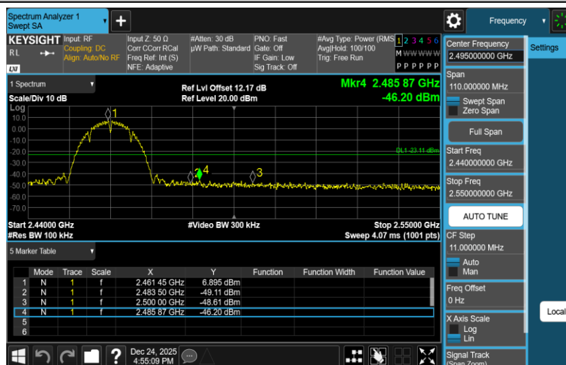
11B-Ant1-2462-PASS
