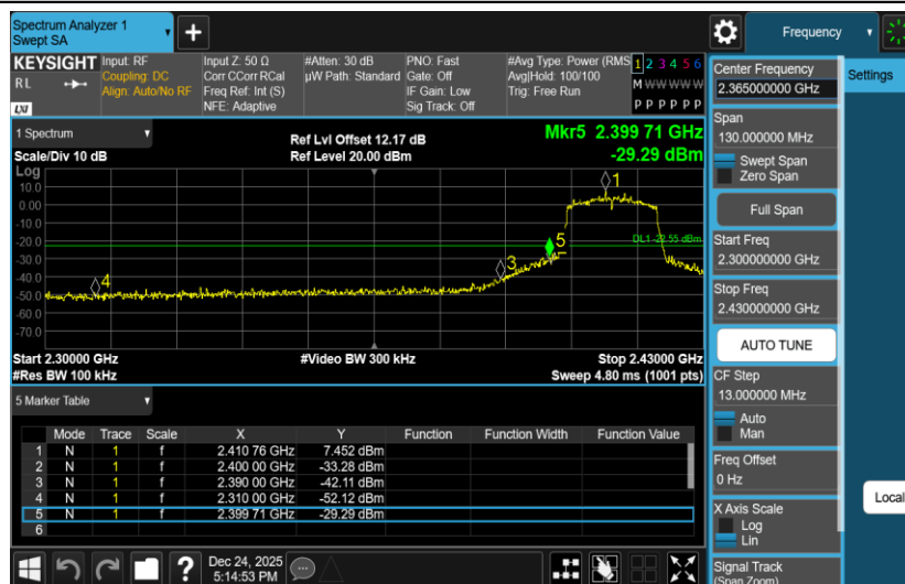
11N20SISO-Ant2-2412-PASS
