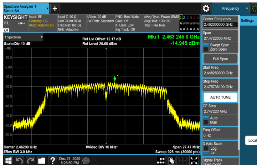
11N20SISO-Ant2-2462-PASS
