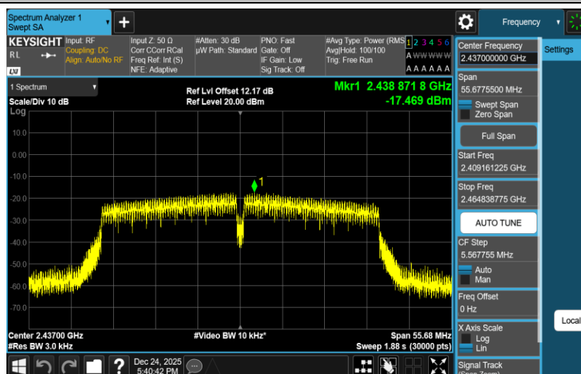
11N40SISO-Ant2-2437-PASS
