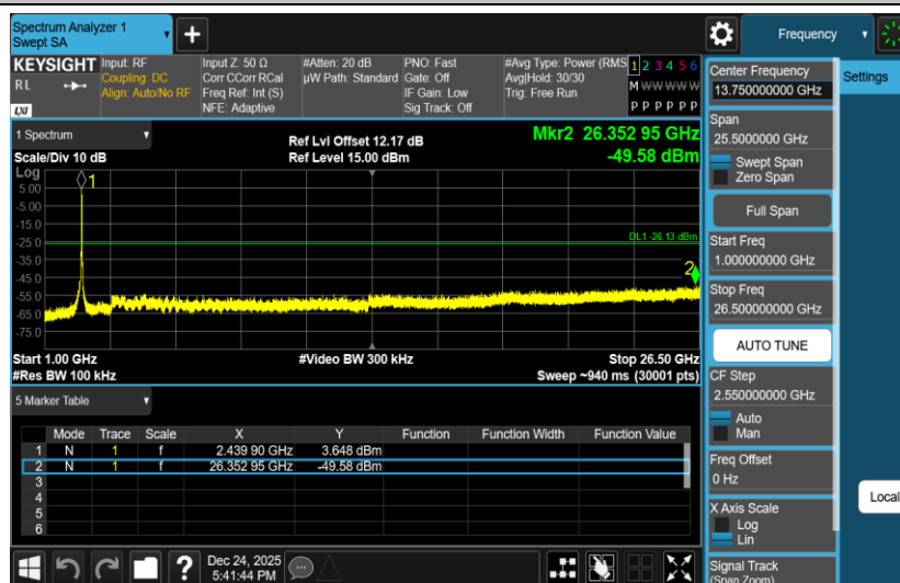
11N40SISO-Ant2-2437-0~Reference-PASS
