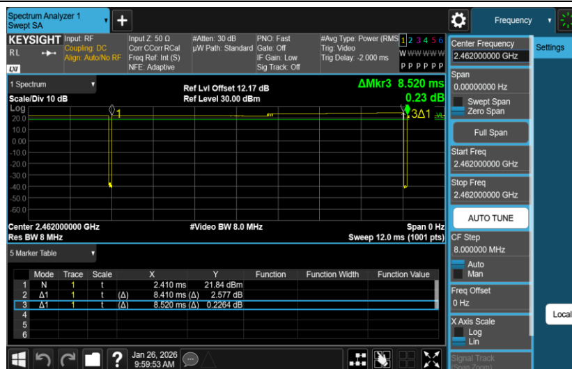
NTNV-11B-Ant2-2462
