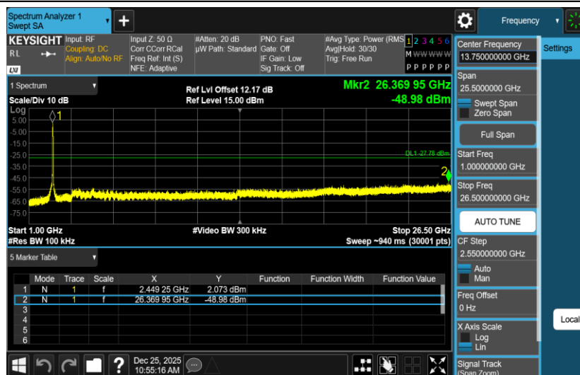
11N40MIMO-Ant2-2452-0~Reference-PASS
