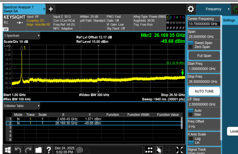
11N40SISO-Ant2-2452-0~Reference-PASS
