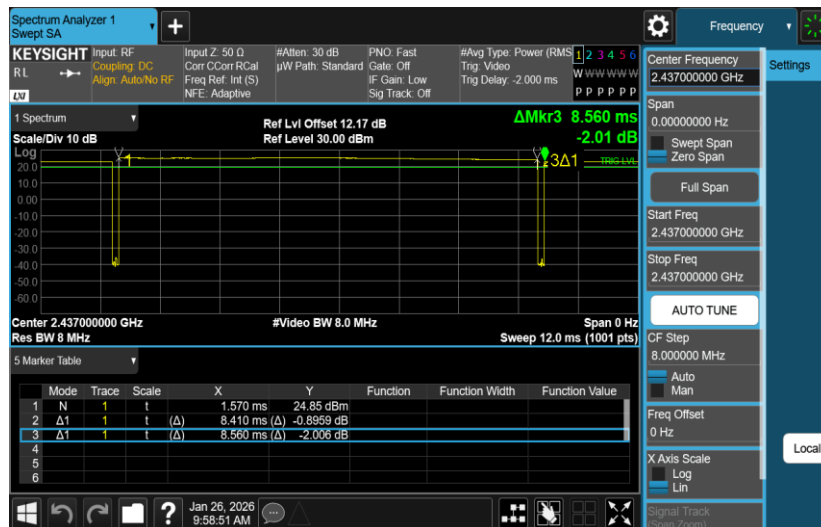
NTNV-11B-Ant2-2437
