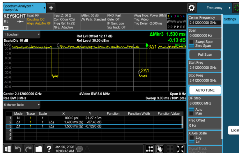
NTNV-11G-Ant2-2412
