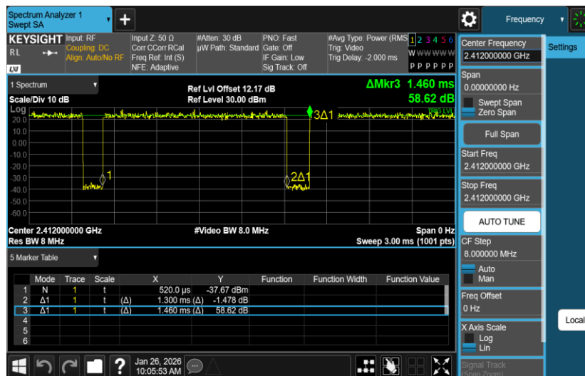
NTNV-11N20SISO-Ant2-2412
