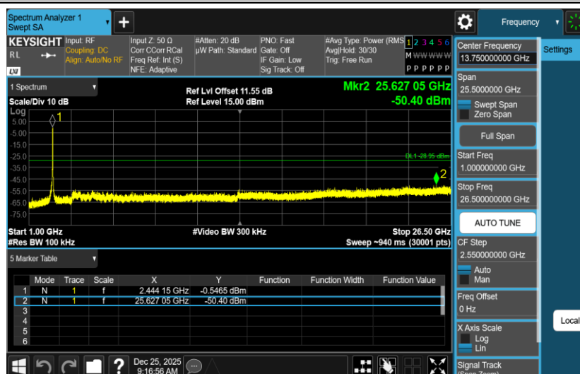
11N40SISO-Ant1-2452-0~Reference-PASS
