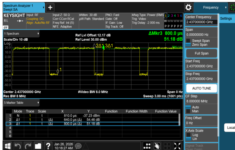
NTNV-11N40SISO-Ant2-2437
