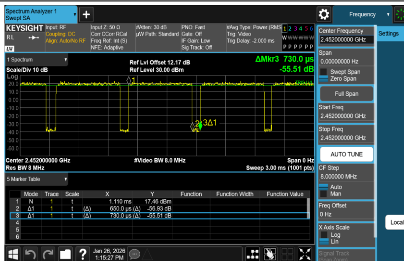
NTNV-11N40MIMO-Ant2-2452
