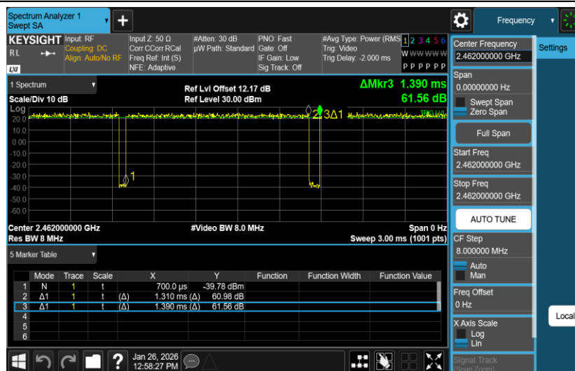
NTNV-11N20MIMO-Ant2-2462
