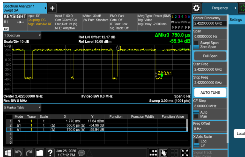
NTNV-11N40MIMO-Ant2-2422
