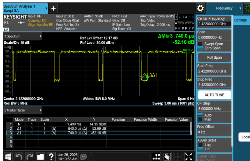
NTNV-11N40SISO-Ant2-2422
