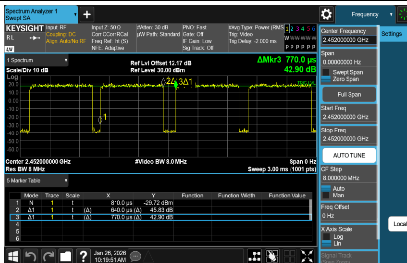
NTNV-11N40SISO-Ant2-2452
