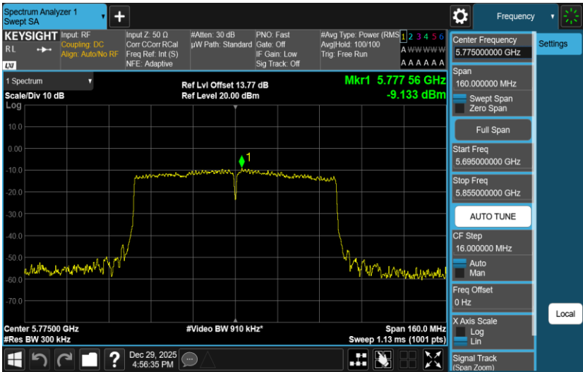
11AC80MIMO-Ant2-5775-PASS
