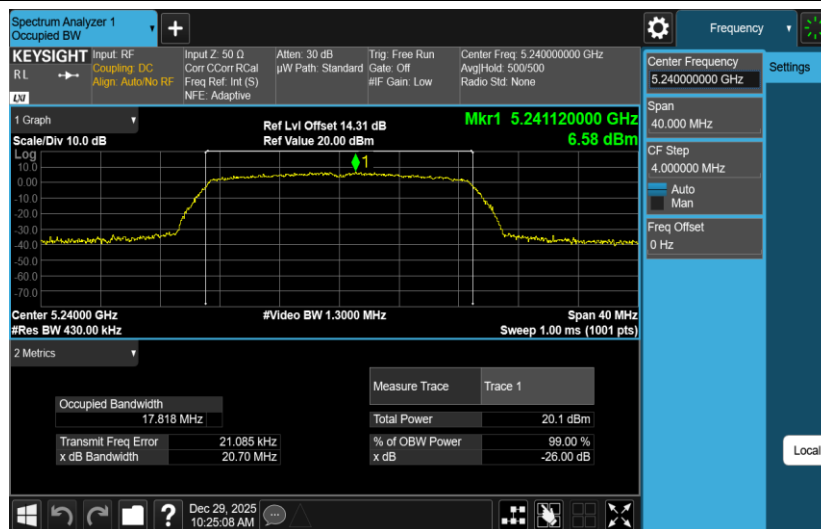
11AC20MIMO-Ant2-5240
