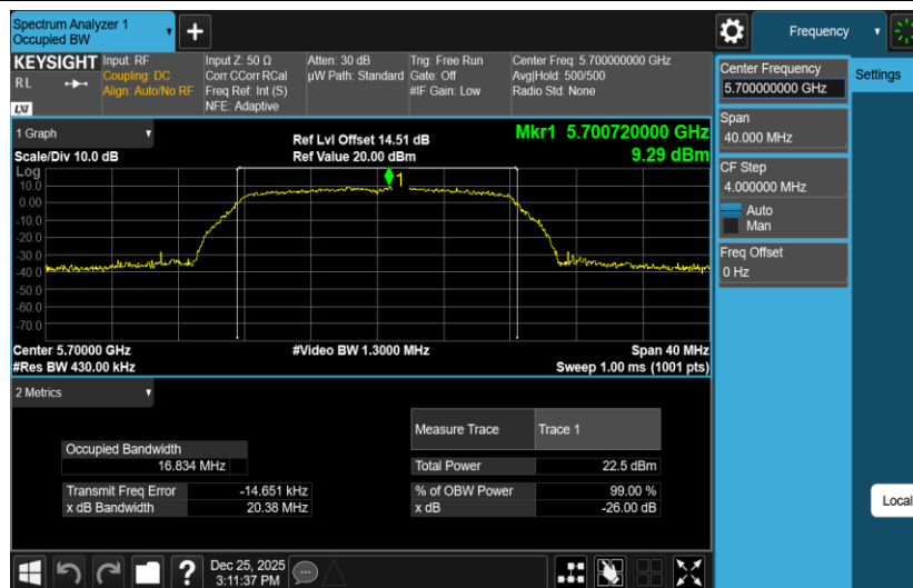
11A-Ant2-5700
