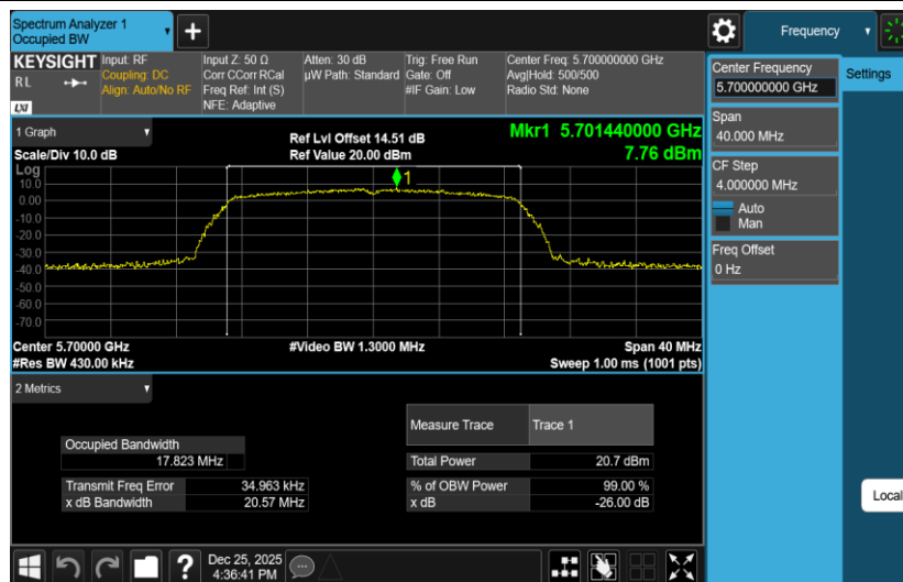
11AC20SISO-Ant2-5700
