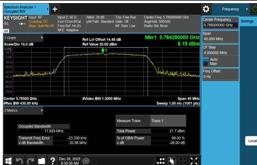
11AC20SISO-Ant2-5785
