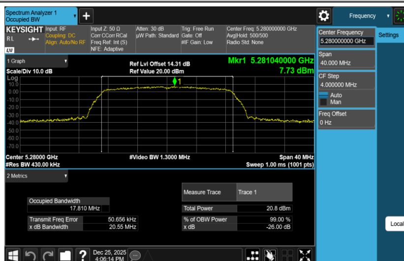
11AC20SISO-Ant2-5280
