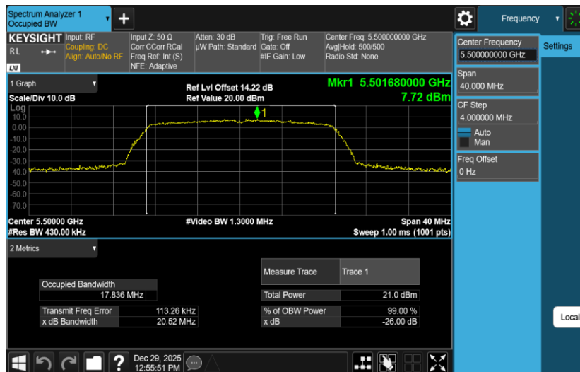
11AC20MIMO-Ant2-5500
