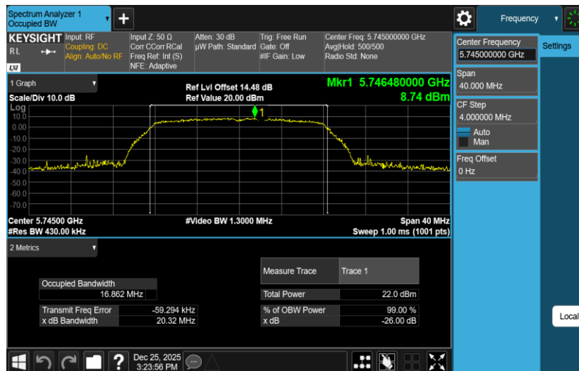
11A-Ant2-5745
