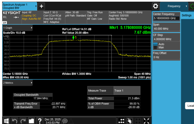
11AC20SISO-Ant2-5180
