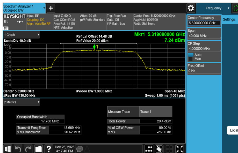
11AC20SISO-Ant2-5320
