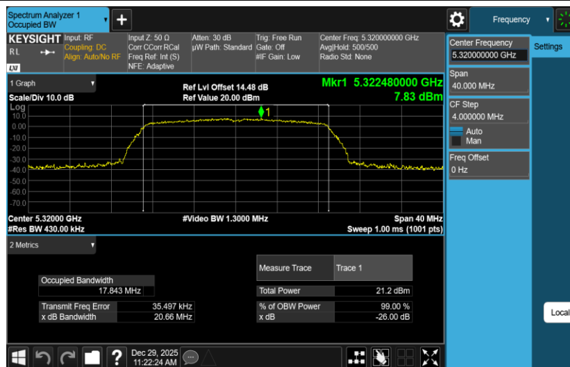
11AC20MIMO-Ant2-5320
