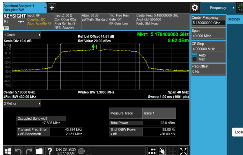
11AC20MIMO-Ant2-5180
