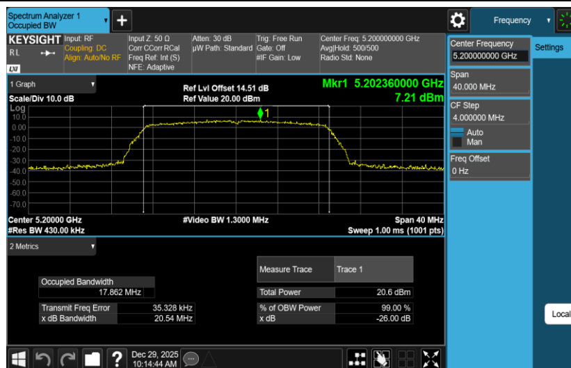
11AC20MIMO-Ant2-5200
