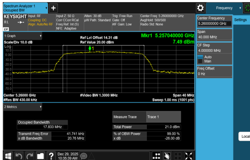
11AC20MIMO-Ant2-5260
