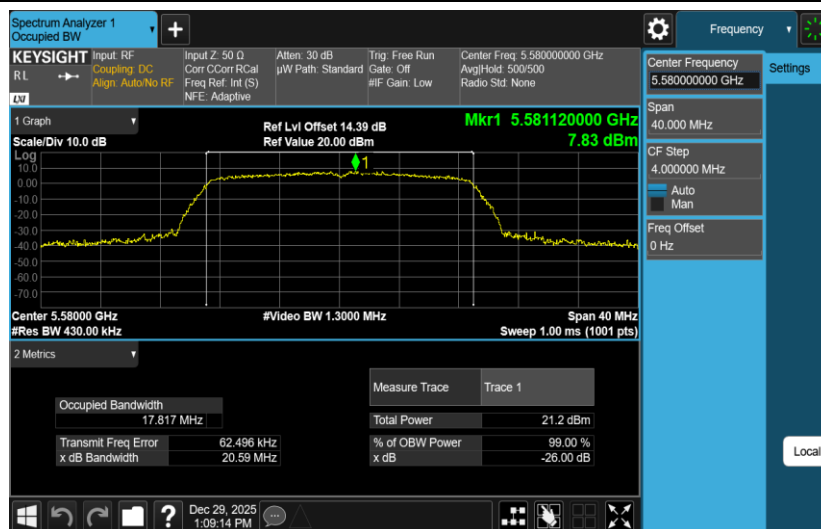
11AC20MIMO-Ant2-5580
