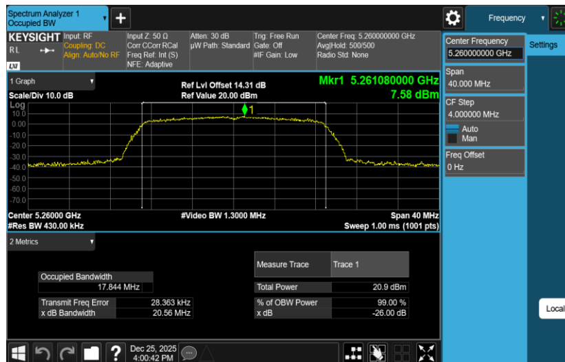
11AC20SISO-Ant2-5260
