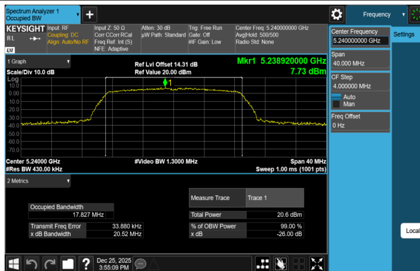
11AC20SISO-Ant2-5240
