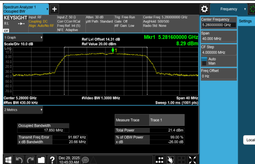
11AC20MIMO-Ant2-5280
