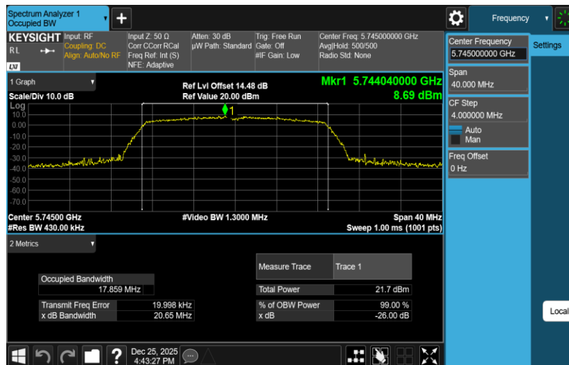
11AC20SISO-Ant2-5745
