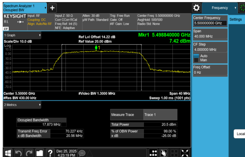
11AC20SISO-Ant2-5500
