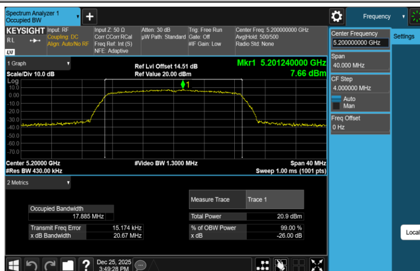
11AC20SISO-Ant2-5200
