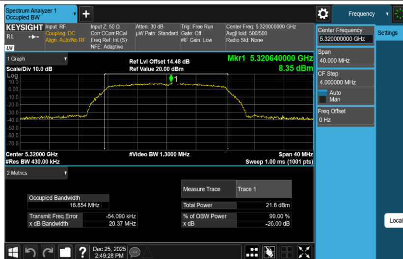
11A-Ant2-5320
