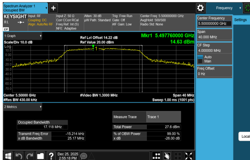
11A-Ant2-5500
