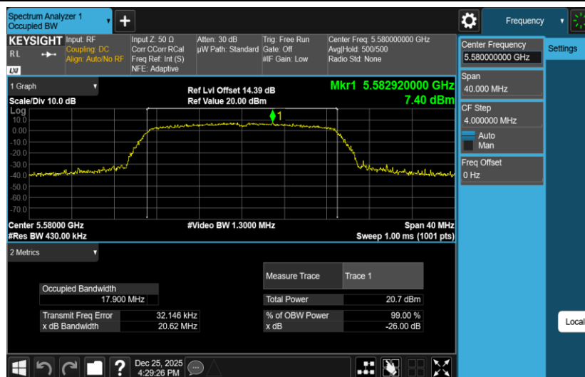
11AC20SISO-Ant2-5580
