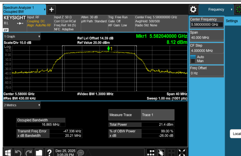
11A-Ant2-5580
