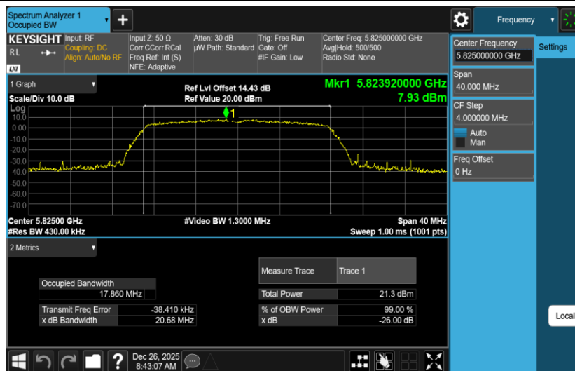
11AC20SISO-Ant2-5825
