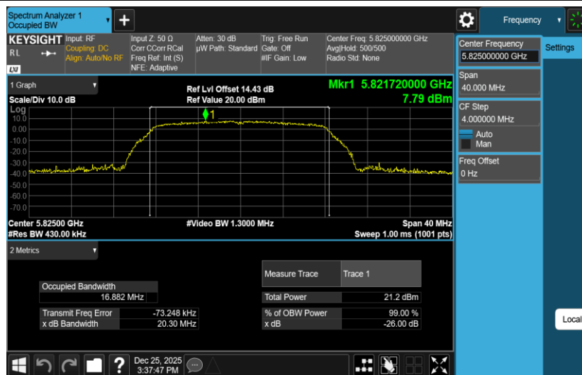
11A-Ant2-5825
