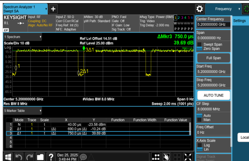
NTNV-11AC20SISO-Ant2-5200
