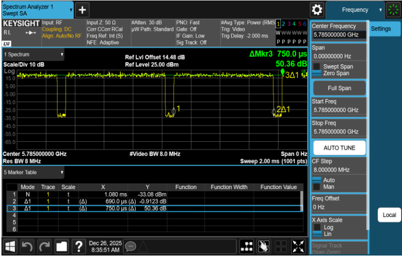
NTNV-11AC20SISO-Ant2-5785
