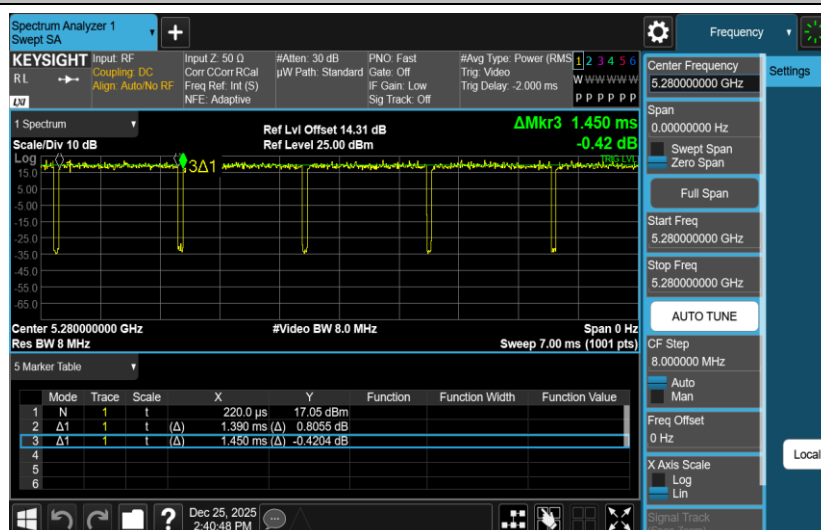
NTNV-11A-Ant2-5280
