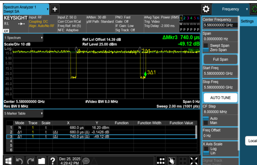
NTNV-11AC20SISO-Ant2-5580
