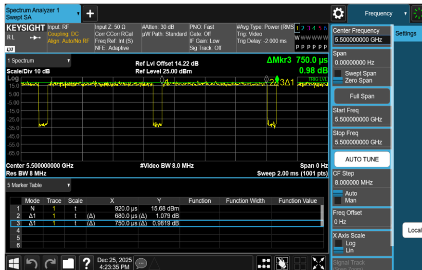
NTNV-11AC20SISO-Ant2-5500
