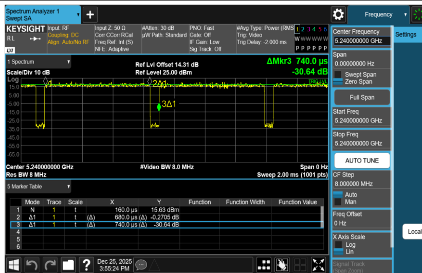
NTNV-11AC20SISO-Ant2-5240
