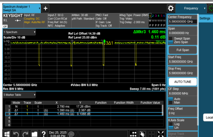
NTNV-11A-Ant2-5580
