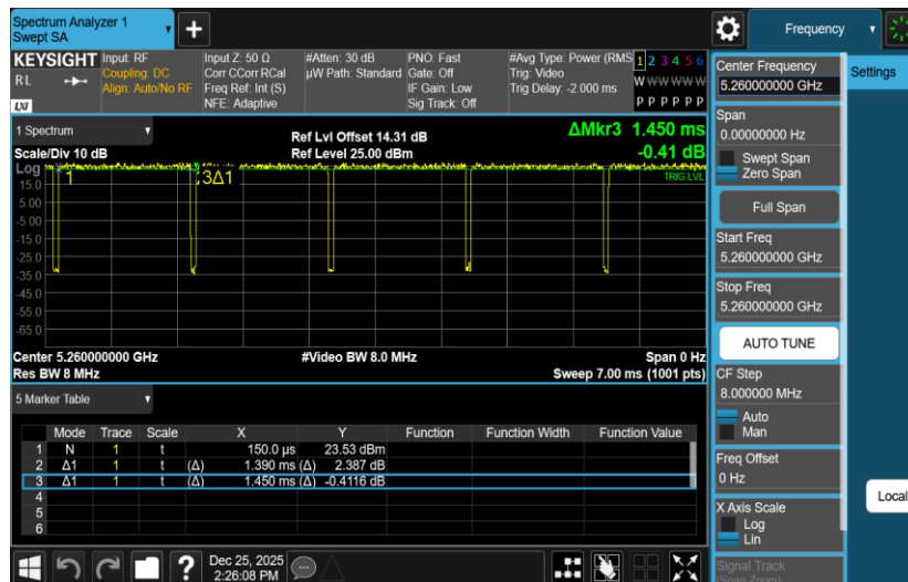
NTNV-11A-Ant2-5260
