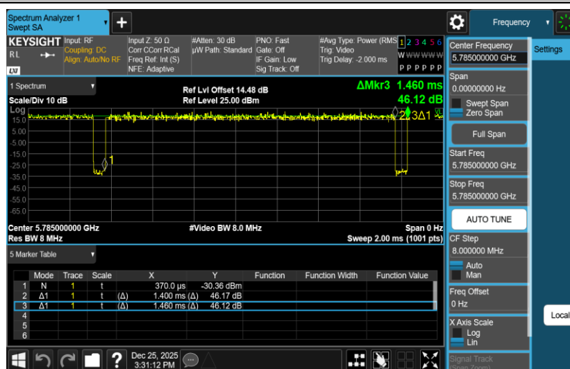
NTNV-11A-Ant2-5785
