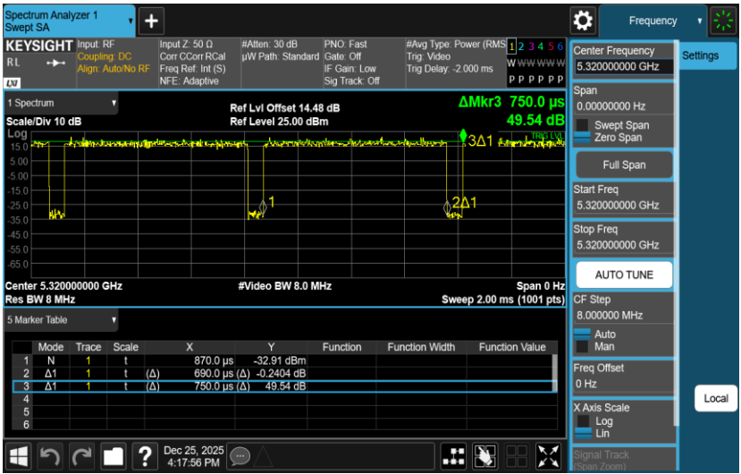
NTNV-11AC20SISO-Ant2-5320
