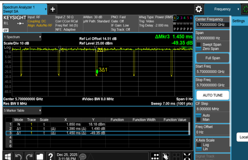
NTNV-11A-Ant2-5700
