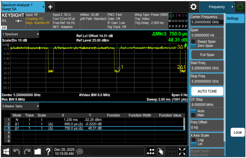
NTNV-11AC20MIMO-Ant2-5200
