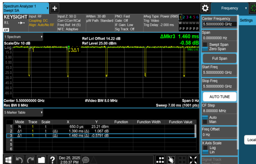
NTNV-11A-Ant2-5500
