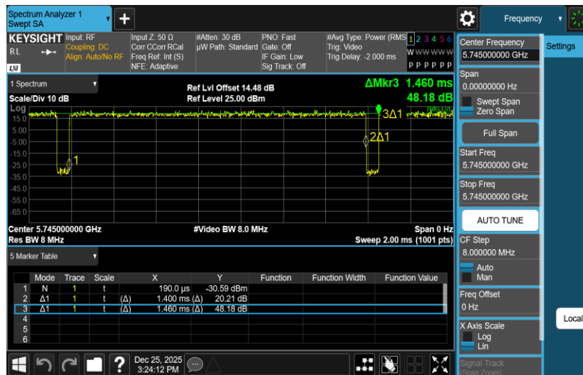
NTNV-11A-Ant2-5745
