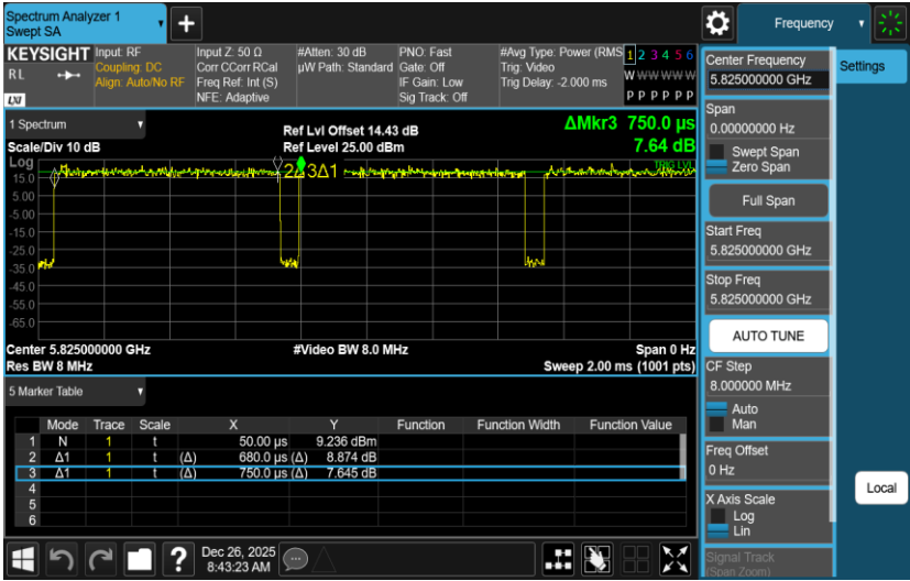
NTNV-11AC20SISO-Ant2-5825
