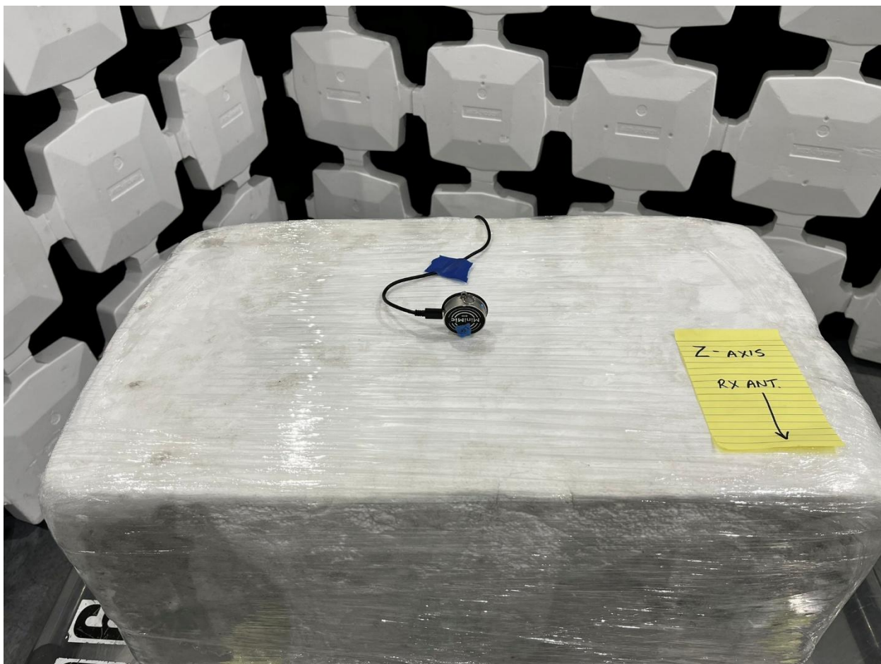
Above 1GHz Radiated Emissions, EUT Z Axis
