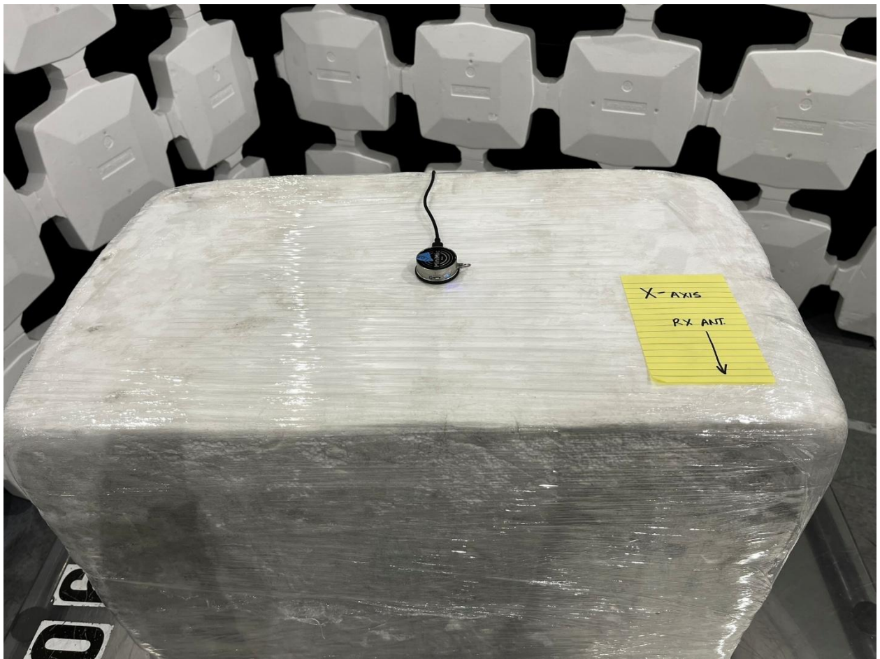
Above 1GHz Radiated Emissions, EUT X Axis
