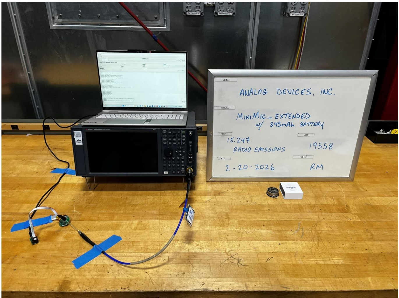
Conducted Radio Emissions, View 1
