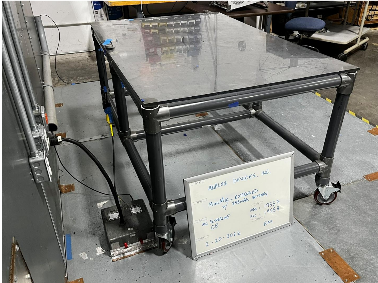
AC Powerline Conducted Emissions, View 2
