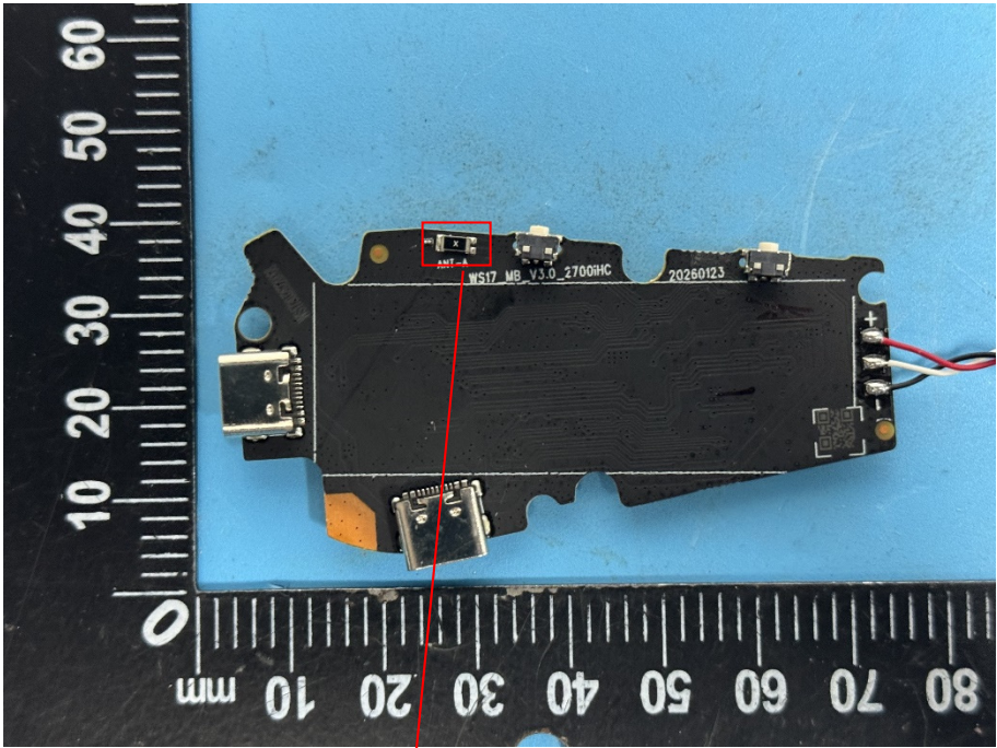
Bluetooth Ant.
