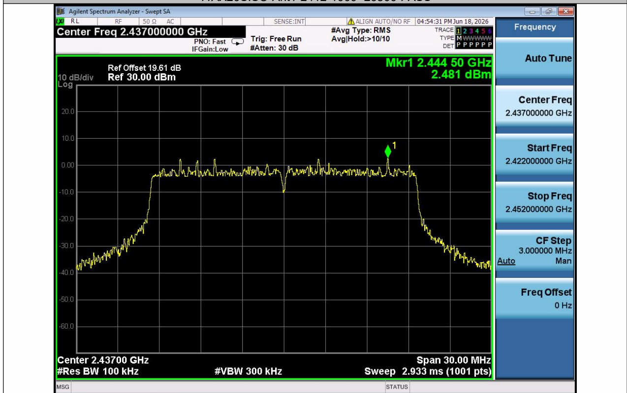
11AX20SISO-Ant1-2437-0~Reference-PASS
