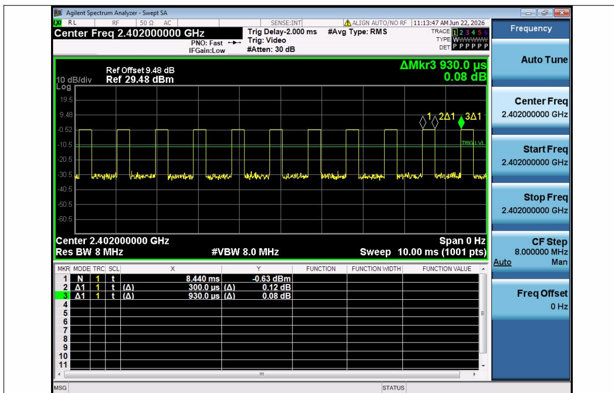
NTNV-BLE_1M-Ant1-2402
