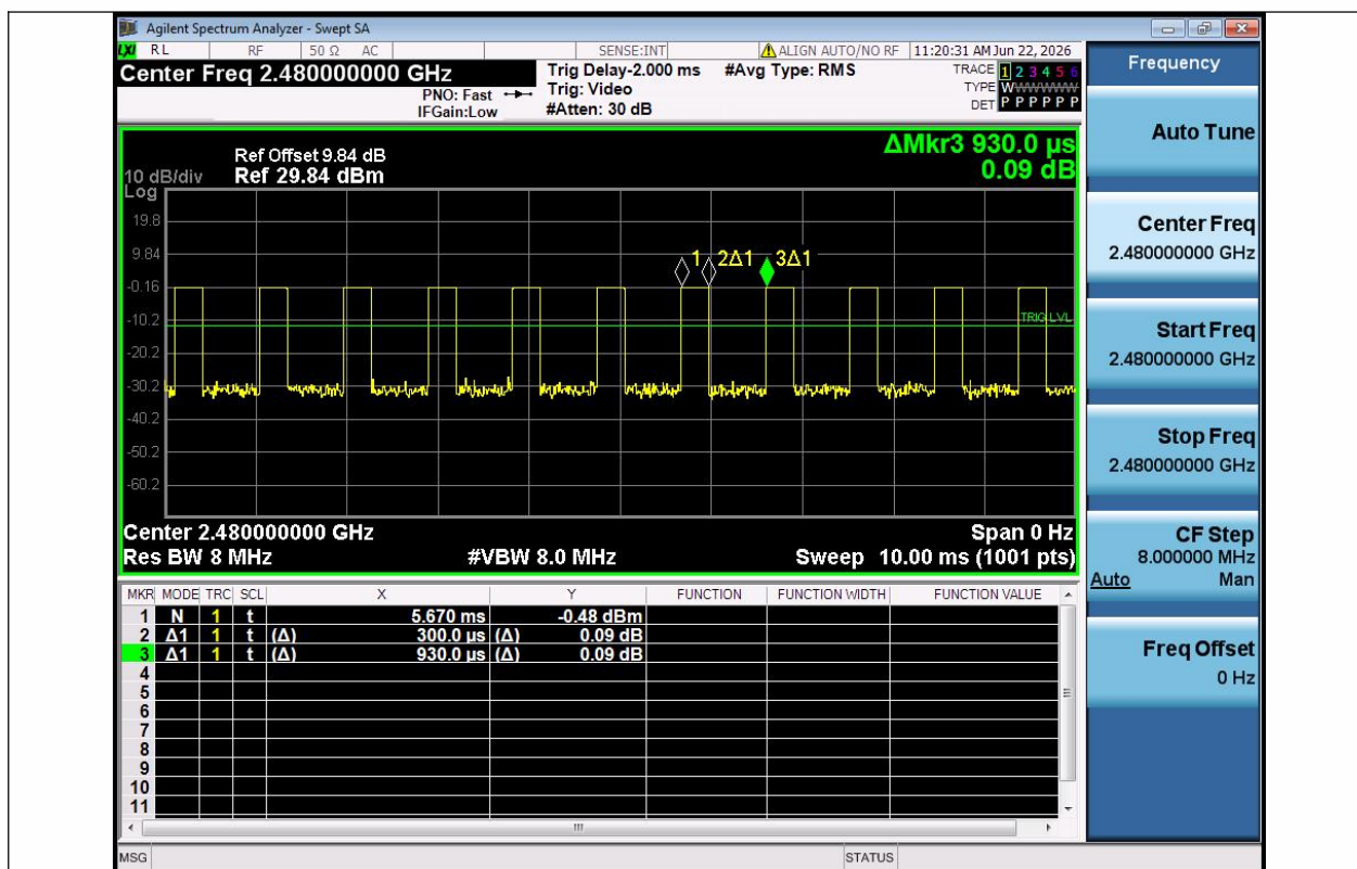
NTNV-BLE_1M-Ant1-2480
