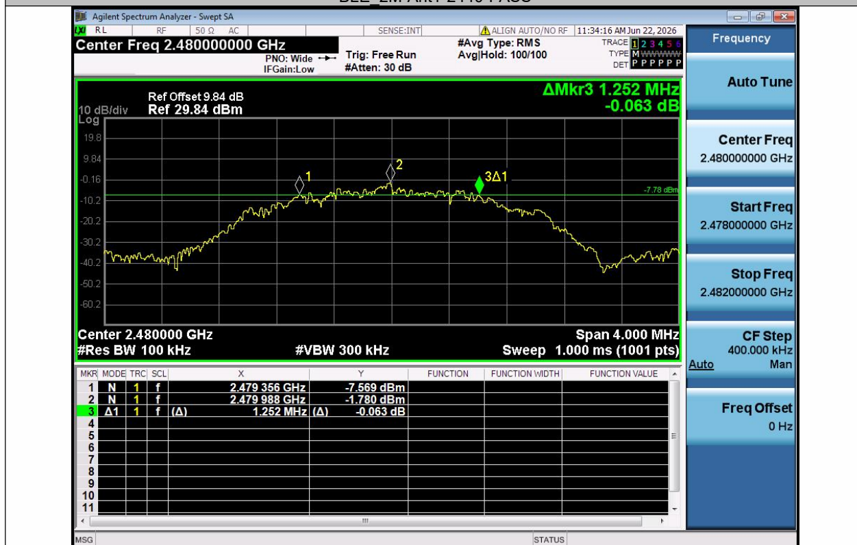
BLE_2M-Ant1-2480-PASS
