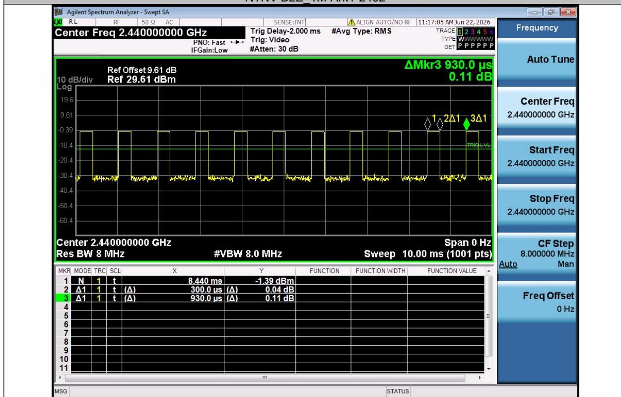
NTNV-BLE_1M-Ant1-2440
