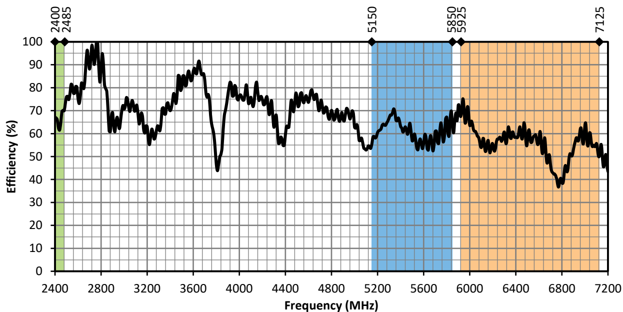
Figure 8: ANT-W63WS5-ccc Antenna Efficiency, Straight
