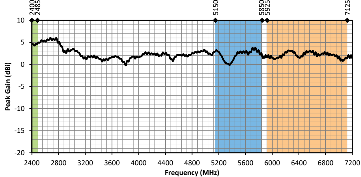
Figure 13: ANT-W63WS5-ccc Peak Gain, Edge-Bent
