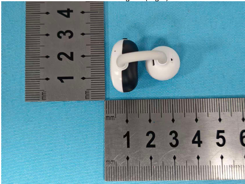
Photo 11 External photos of EUT Smart Hearing Aid (Right)
