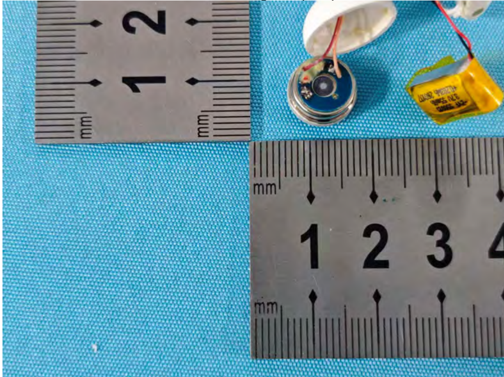
Photo 5 Internal photos of EUT Smart Hearing Aid (Left)
