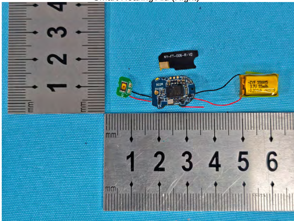
Photo 12 Internal photos of EUT Smart Hearing Aid (Right)
