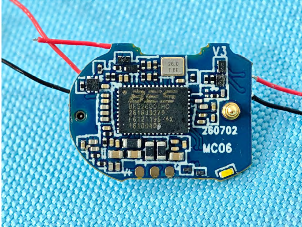
Photo 17 Internal photos of EUT Smart Hearing Aid (Right)
