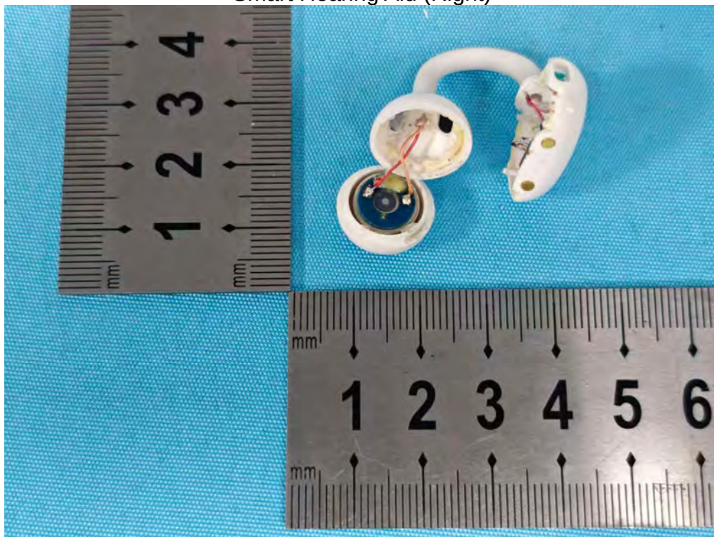
Photo 14 Internal photos of EUT Smart Hearing Aid (Right)
