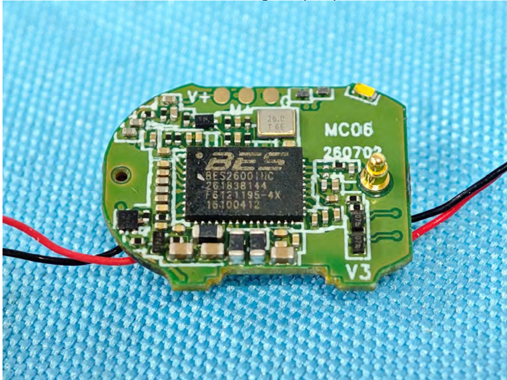
Photo 7 Internal photos of EUT Smart Hearing Aid (Left)
