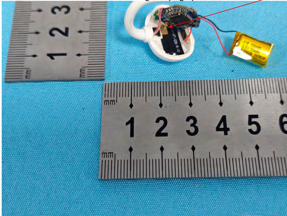
Photo 11 Internal photos of EUT Smart Hearing Aid (Right)
