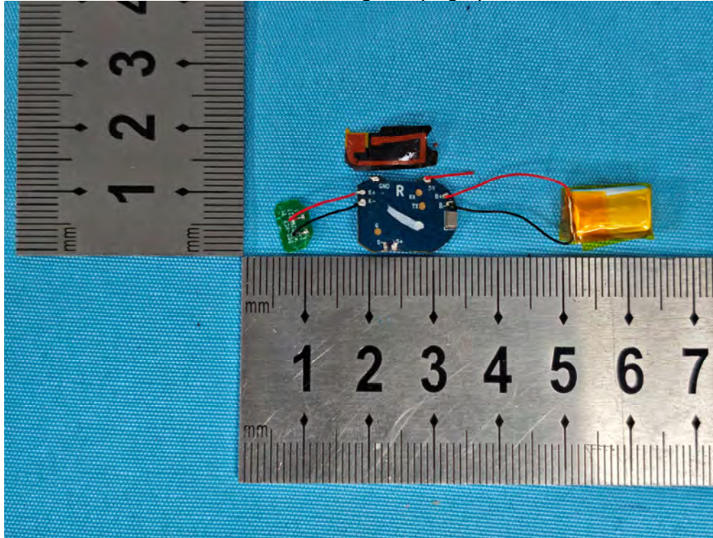
Photo 13 Internal photos of EUT Smart Hearing Aid (Right)
