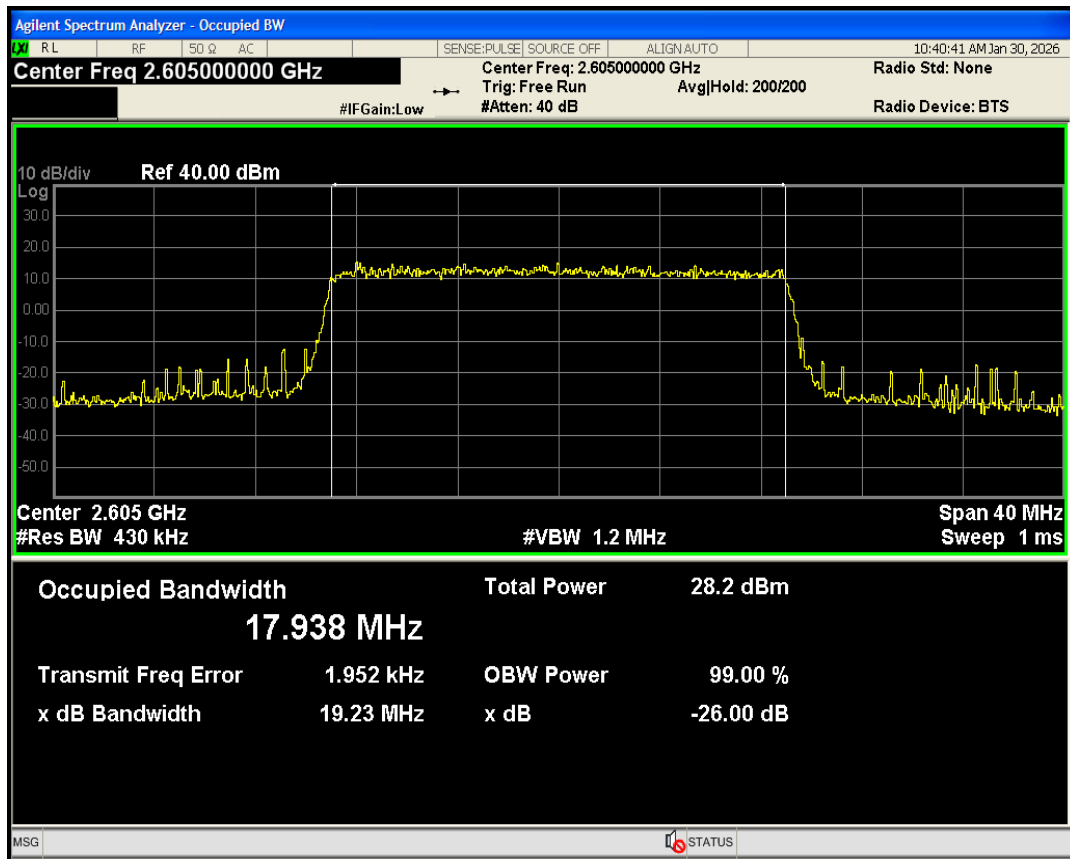
Band41(2535-2675) QAM16 BW=20MHz Channel=40740 RB Size=100 Position=#0
