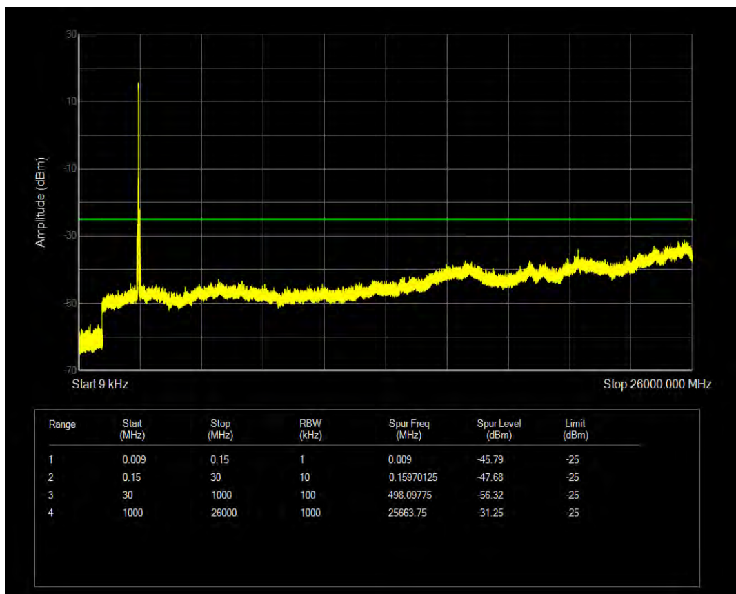
Band41(2535-2675) QPSK BW=20MHz Channel=40140 RB Size=100 Position=#0
