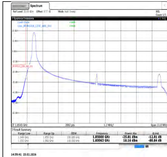
Band25-10MHz-16QAM-26090-50RB#0-PASS
