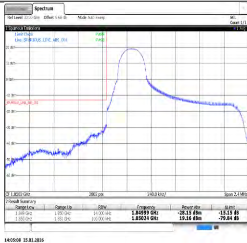
Band25-1.4MHz-QPSK-26047-6RB#0-PASS
