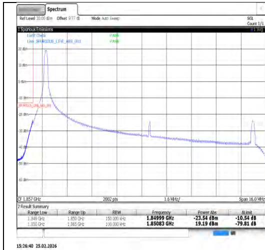
Band25-15MHz-QPSK-26115-75RB#0-PASS
