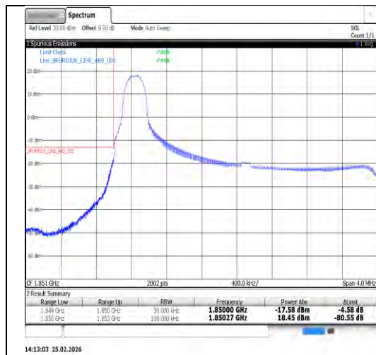
Band25-3MHz-16QAM-26055-15RB#0-PASS
