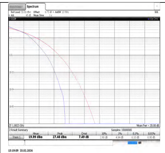
Band25-15MHz-16QAM-26365-75RB#0-PASS
