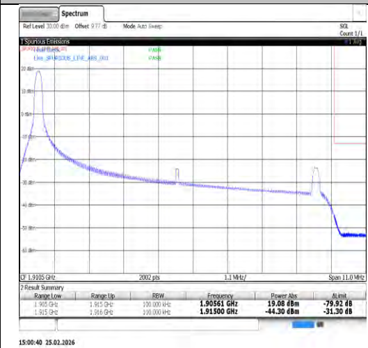
Band25-10MHz-16QAM-26640-50RB#0-PASS
