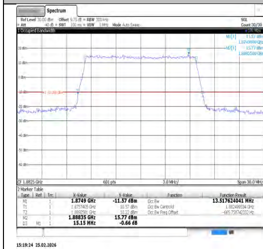
Band25-15MHz-QPSK-26365-75RB#0-PASS
