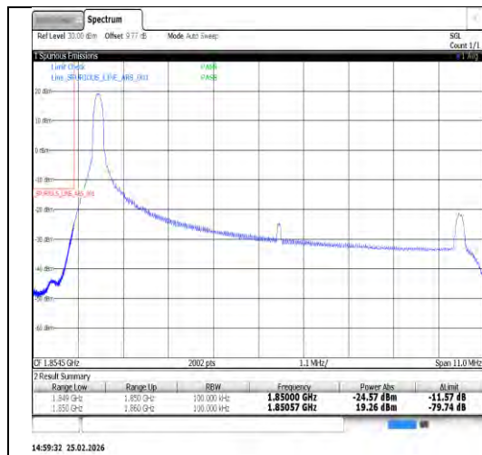
Band25-10MHz-QPSK-26090-50RB#0-PASS
