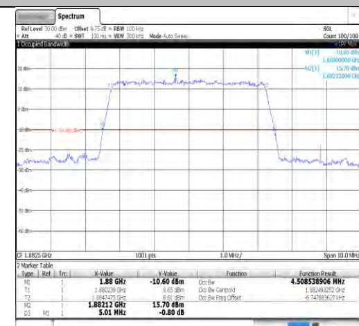
Band25-5MHz-16QAM-26365-25RB#0-PASS
