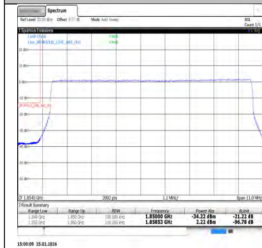
Band25-10MHz-QPSK-26640-1RB#49-PASS
