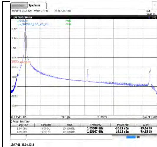
Band25-20MHz-QPSK-26140-100RB#0-PASS
