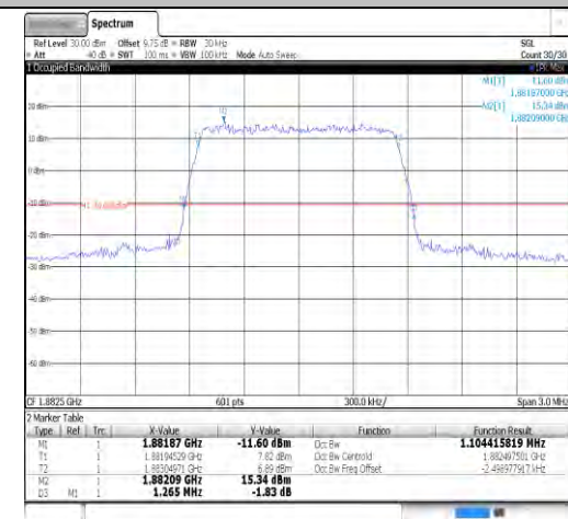
Band25-1.4MHz-16QAM-26365-6RB#0-PASS
