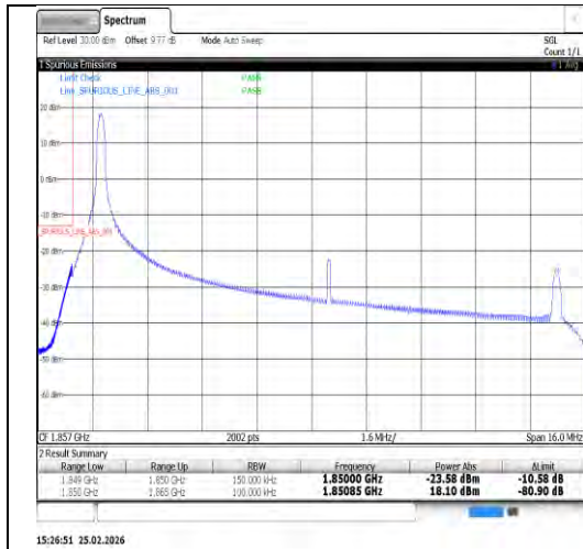
Band25-15MHz-16QAM-26115-75RB#0-PASS
