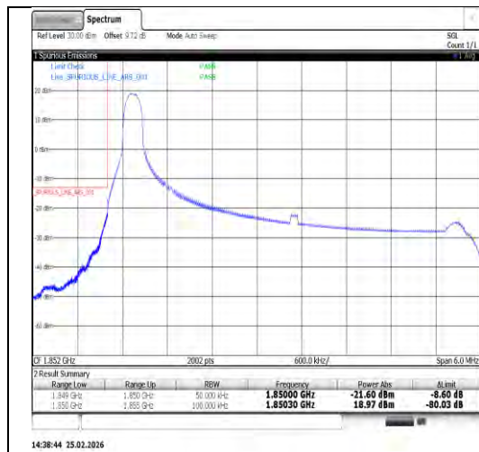
Band25-5MHz-QPSK-26065-25RB#0-PASS
