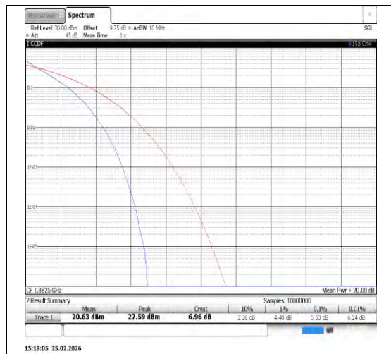
Band25-15MHz-QPSK-26365-75RB#0-PASS
