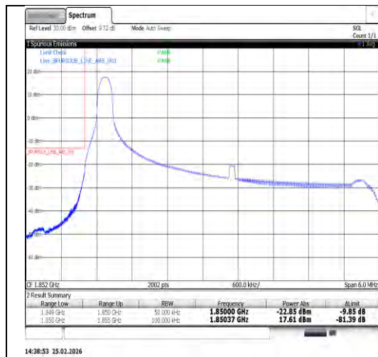
Band25-5MHz-16QAM-26065-25RB#0-PASS
