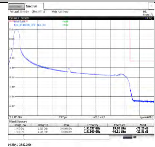
Band25-5MHz-QPSK-26665-25RB#0-PASS
