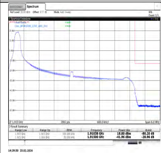
Band25-5MHz-16QAM-26665-25RB#0-PASS
