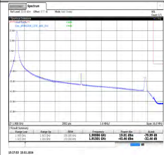
Band25-15MHz-16QAM-26615-75RB#0-PASS
