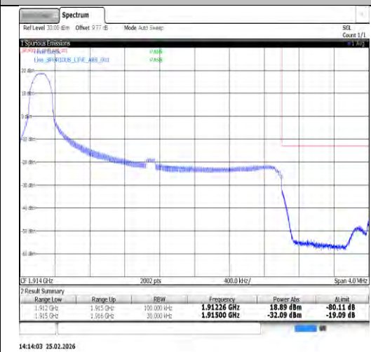
Band25-3MHz-16QAM-26675-15RB#0-PASS
