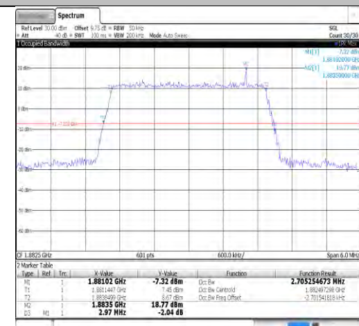
Band25-3MHz-16QAM-26365-15RB#0-PASS
