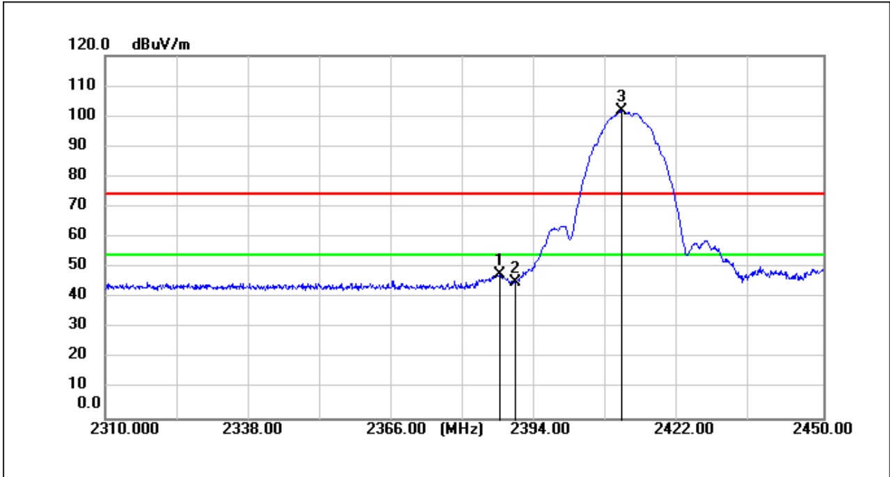
11b_TX_CH_01_Vertical_Peak
