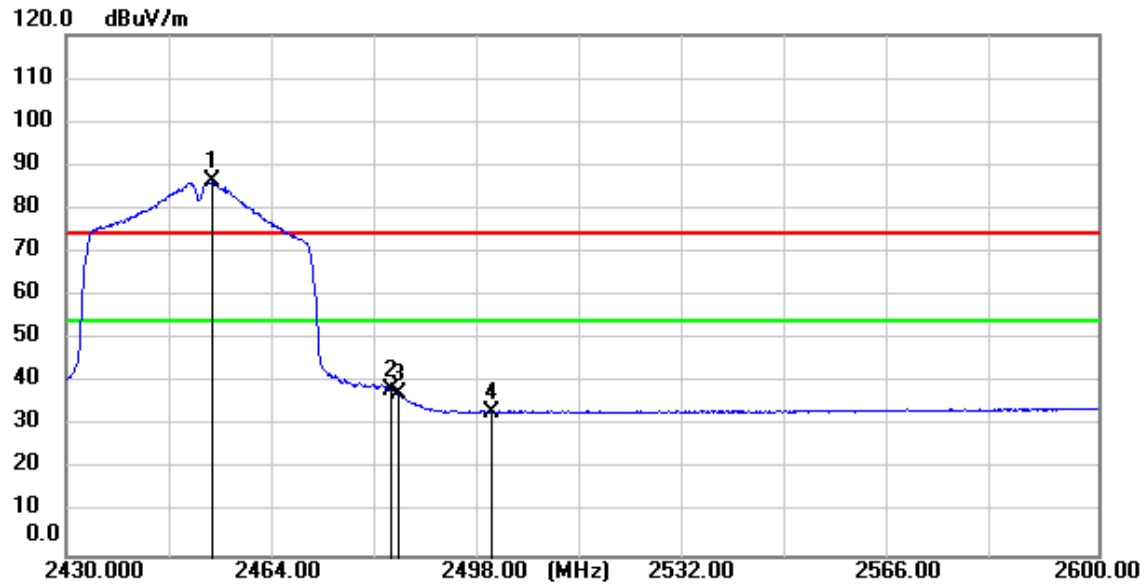
11n(HT40)_TX_CH_09_Vertical_Average
