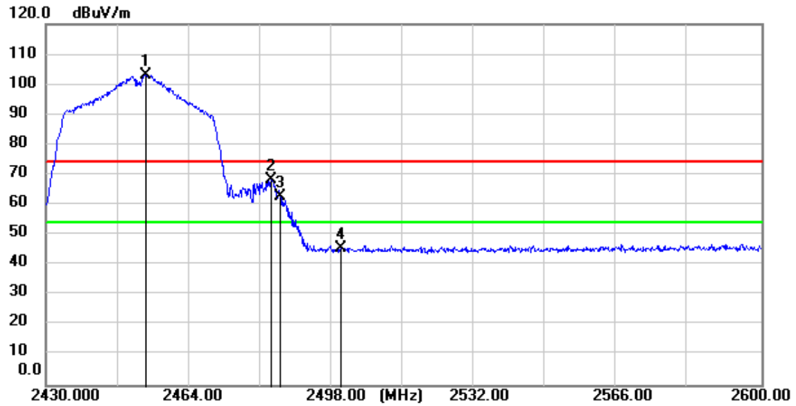
11n(HT40)_TX_CH_09_Horizontal_Peak
