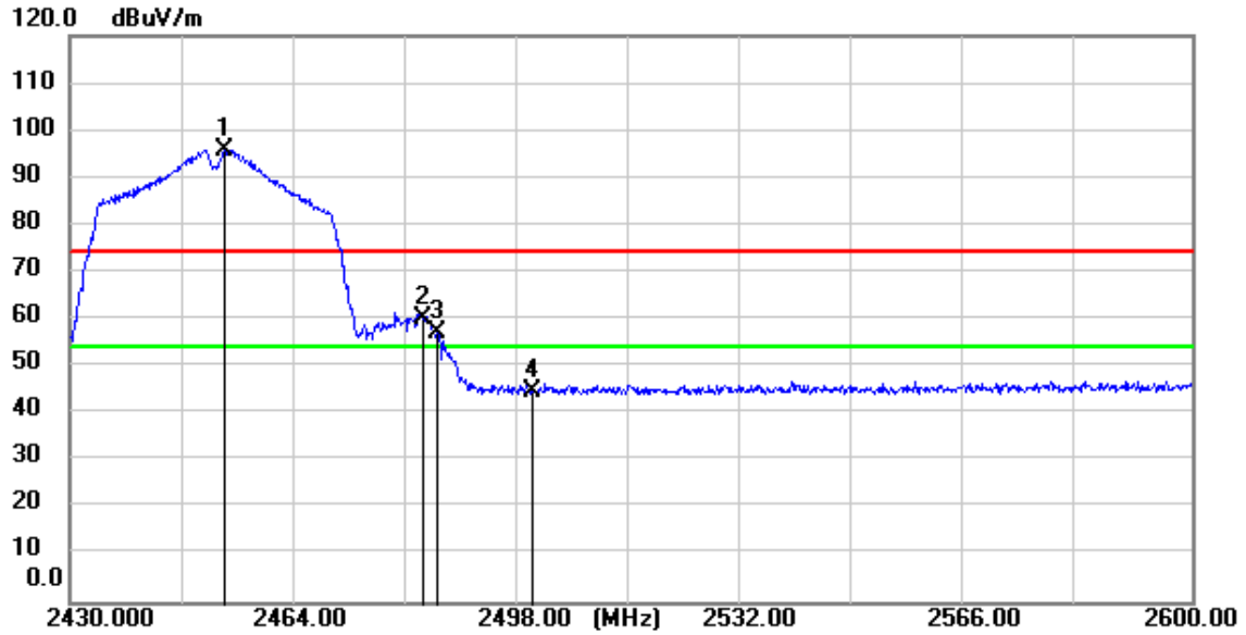
11n(HT40)_TX_CH_09_Vertical_Peak
