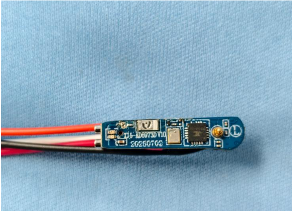
Internal Photo (Left ear plug)
