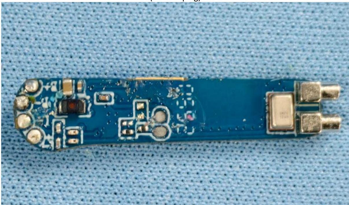
Internal Photo (Left ear plug)
