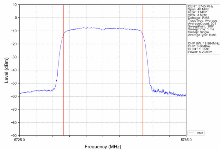
802.11ax(HEW20)_LCH_5745MHz_SU_/_Ant1_NTNV
