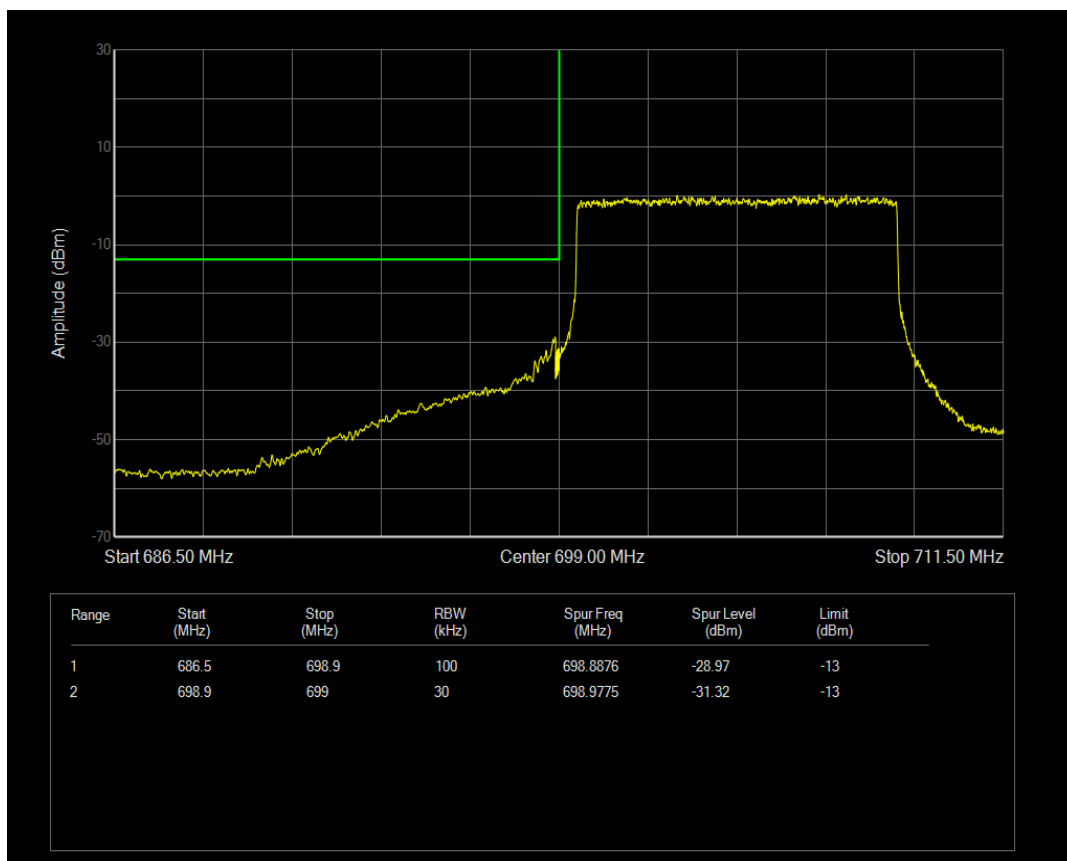
Band12 QAM16 BW=10MHz Channel=23060 RB Size=27 Position=#0
