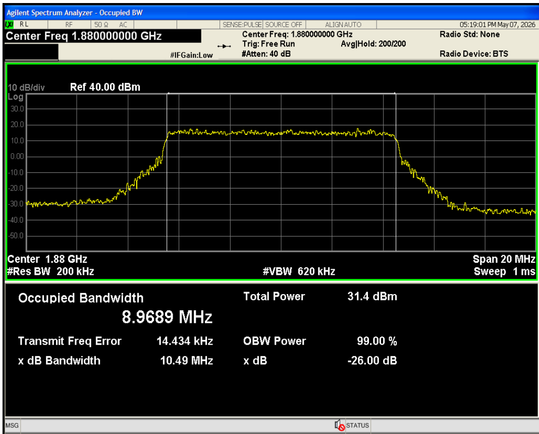
Band2 QAM16 BW=10MHz Channel=18900 RB Size=27 Position=#0
