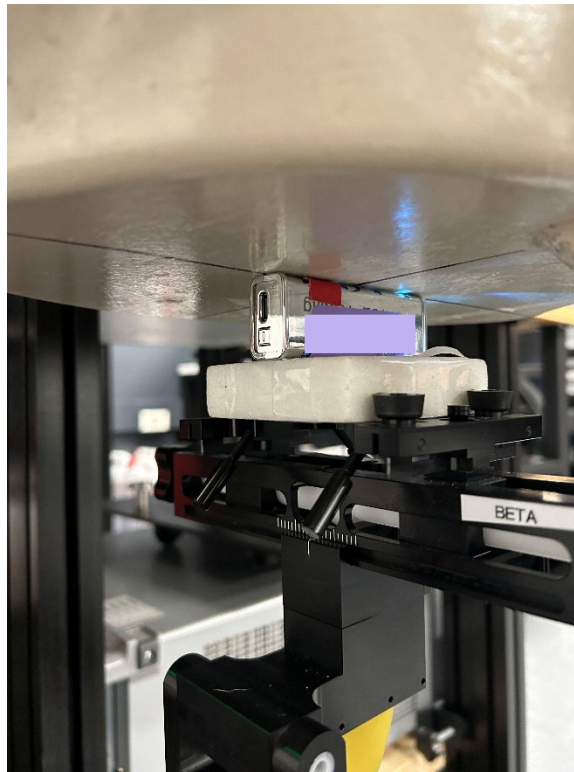
Figure 5 SAR Test Setup – Body/Extremity – Right Edge 0mm
