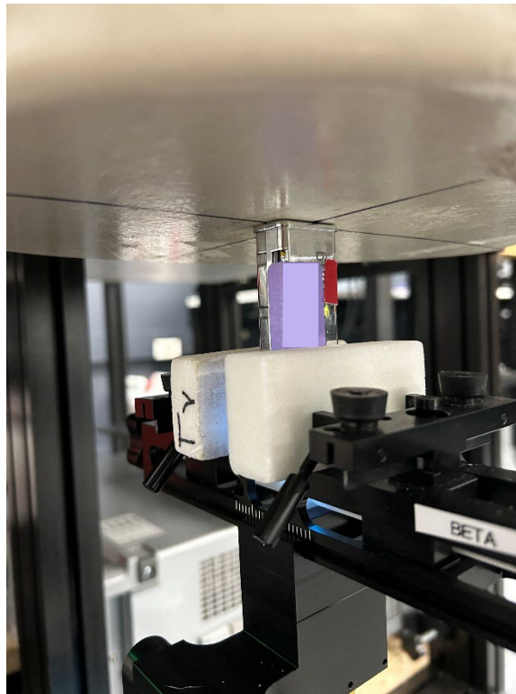
Figure 3 SAR Test Setup – Body/Extremity – Top Edge 0mm
