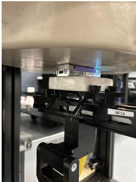
Figure 2 SAR Test Setup – Body/Extremity – Front Side 0mm
