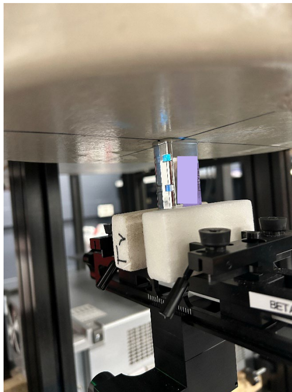
Figure 4 SAR Test Setup – Body/Extremity – Bottom Edge 0mm
