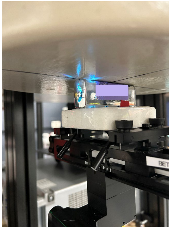
Figure 6 SAR Test Setup – Body/Extremity – Left Edge 0mm
