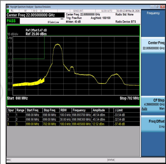
Band12-3MHz-QPSK-23025-PASS
