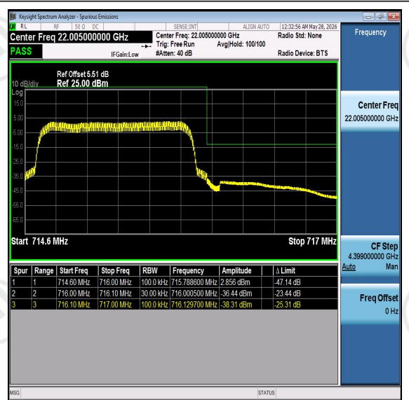
Band12-1.4MHz-16QAM-23173-PASS
