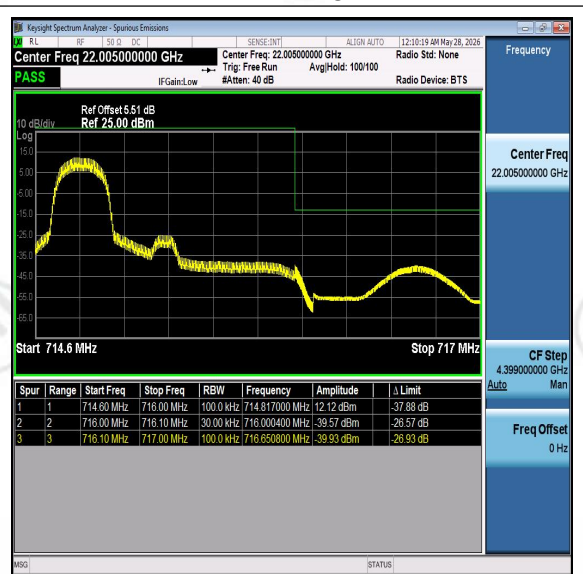
Band12-1.4MHz-16QAM-23173-PASS
