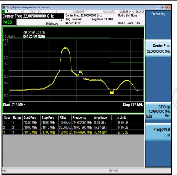
Band12-3MHz-16QAM-23165-PASS
