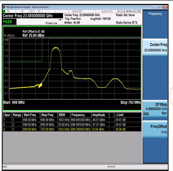
Band12-3MHz-16QAM-23025-PASS
