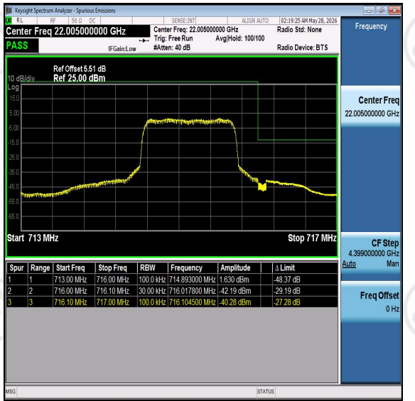
Band12-3MHz-16QAM-23165-PASS
